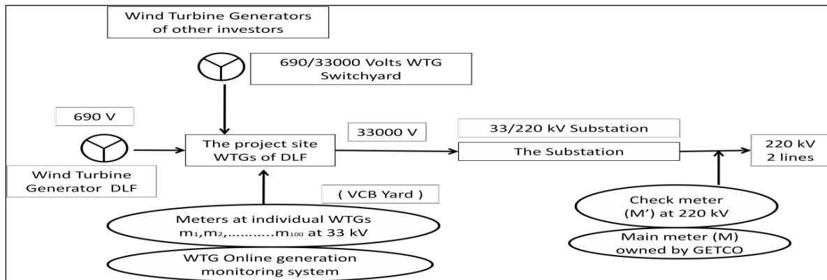
Figure: The wire diagram for the meters at substation:
