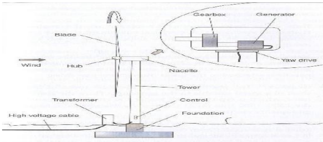
Figure 2: Cross sectional diagram of wind turbine
