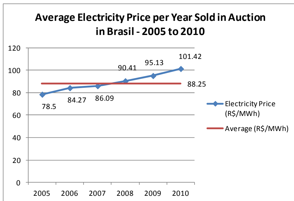
Figure 1: Average electricity Price sold in Auctions in Brasil from 2005 to 2010
