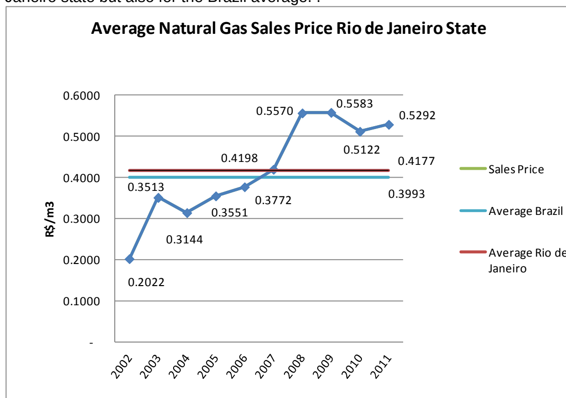
Figure 2: Reference price for natural gas in Rio de Janeiro state and Brasil from 2003 to 2011
