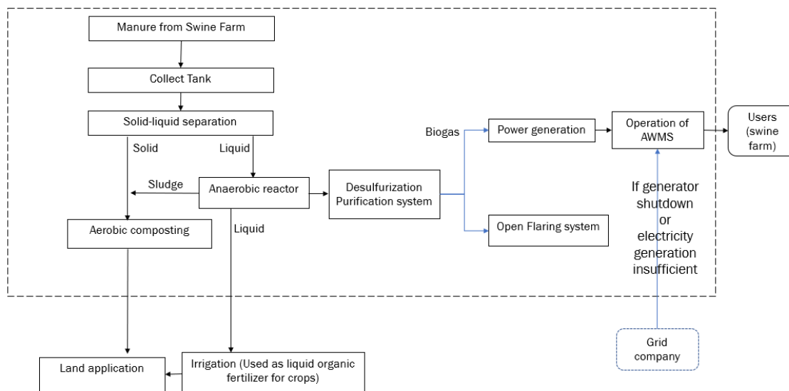
Figure 3-1 Process flow diagram of the project activity
