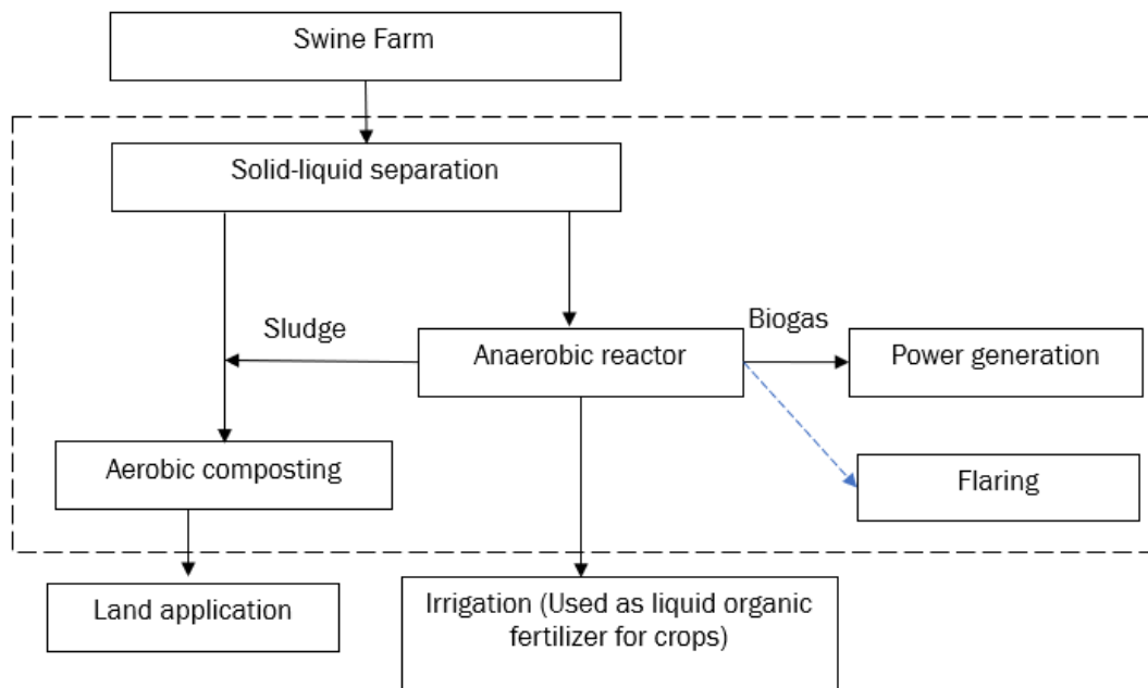
Figure 1-1 Process flow diagram of the project activity
