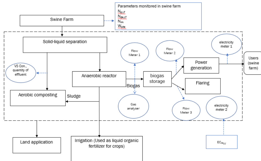
Figure 5-2 Installation and Configuration of Meters
