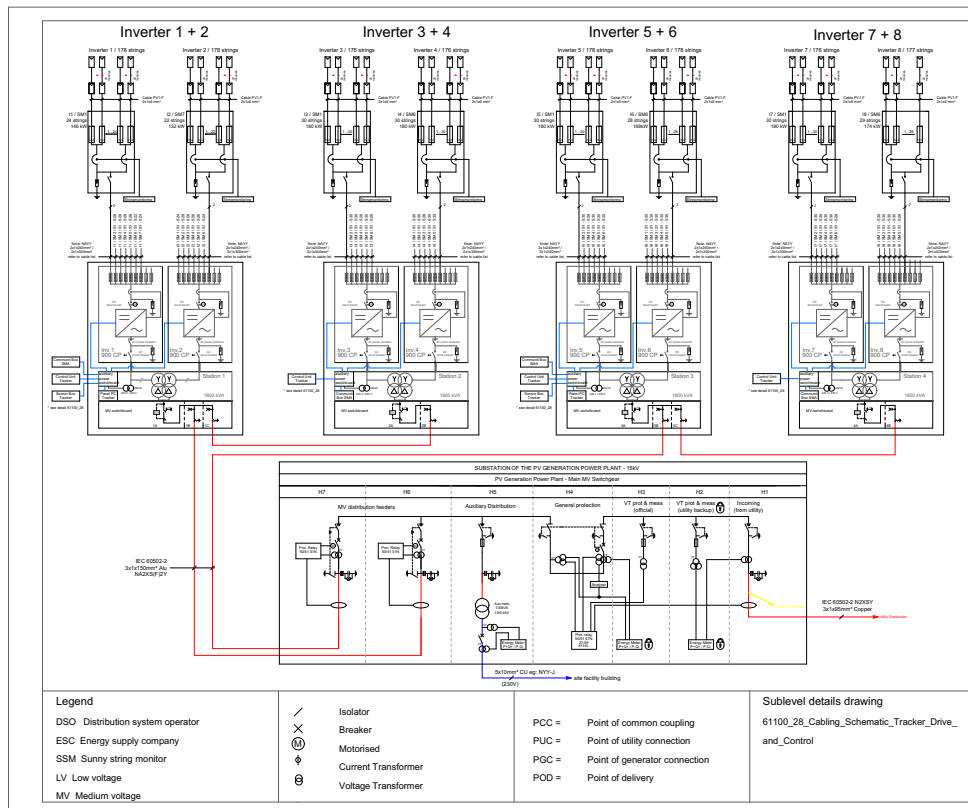
Figure 2: Schematic layout of the power plant
