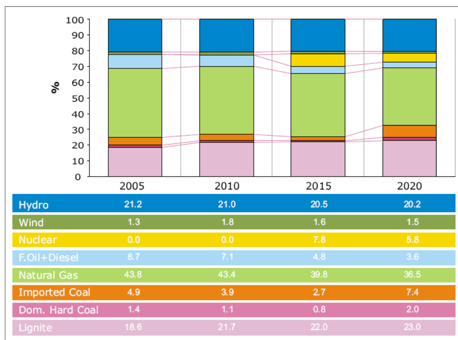
Figure 3. Electricity Generation Forecast (2008-2017)
