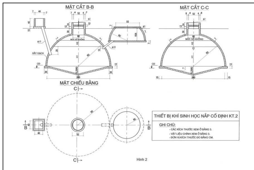
Figure 6: KT2B biogas plant example design
