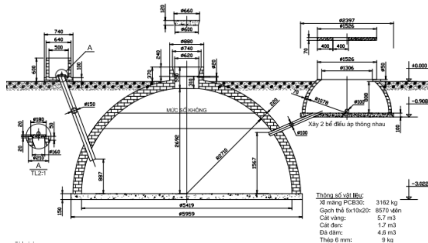
Figure 5: KT2 (or KT2A) biogas plant example design
