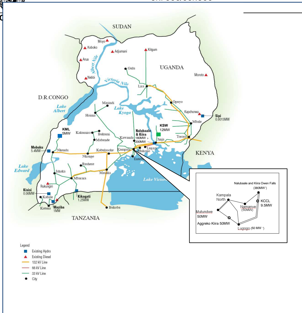
Figure 7: Uganda national electricity grid
