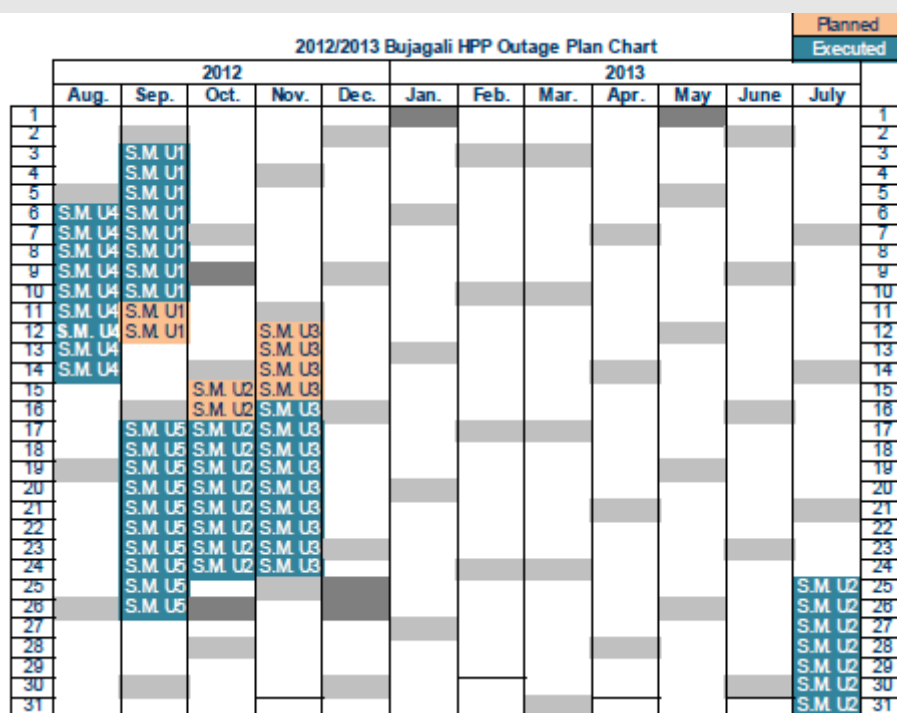
Figure 4: Bujagali HPP Outage Plan Chart August 2012 - July 2013
