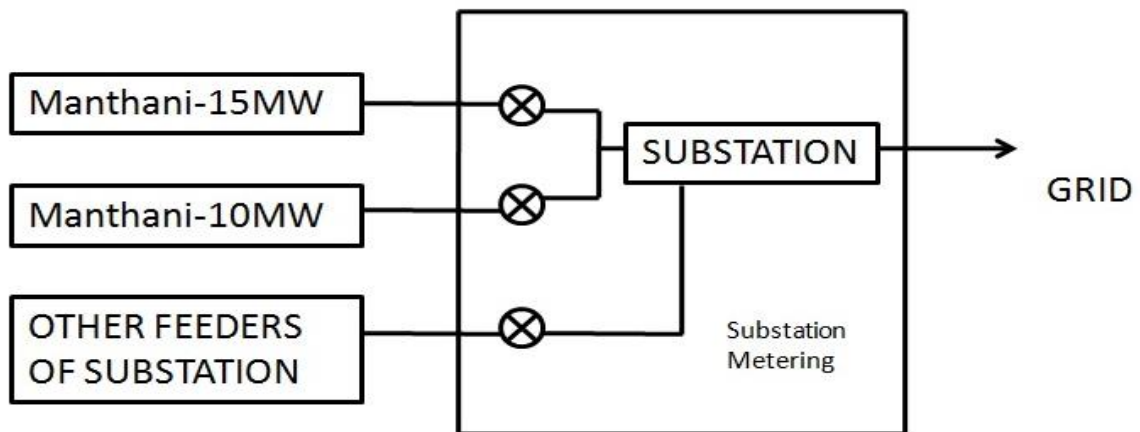
Figure 14 Line diagram of Purvanchal Solar Power Pvt. Ltd.
