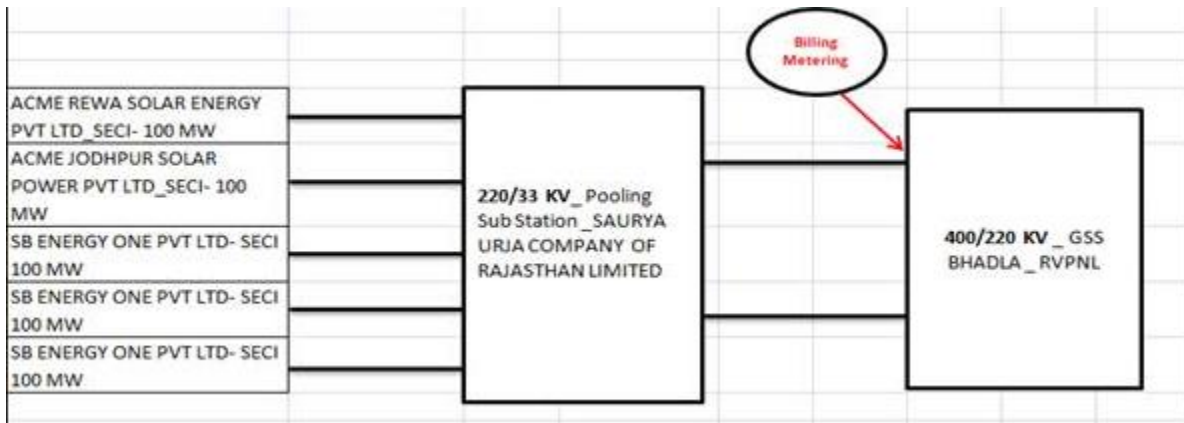
Figure 12 Line diagram of ACME Rewa Solar Energy Pvt. Ltd.
