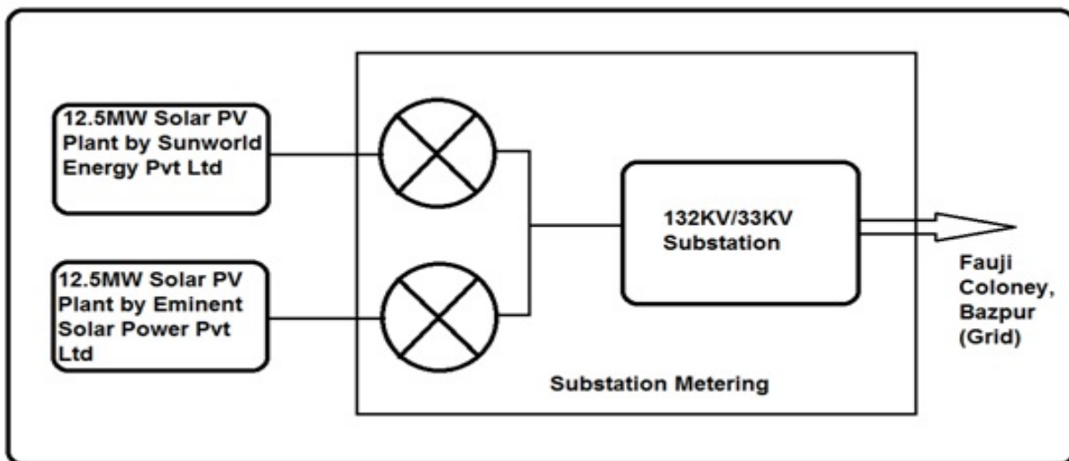
Figure 22 Line diagram of Sunworld Energy Pvt. Ltd.
