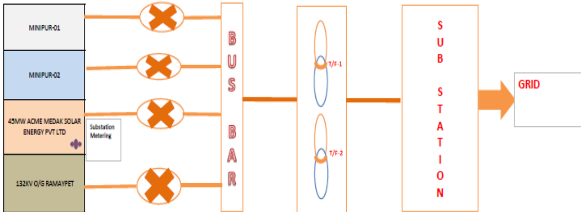
Figure 4 Line diagram of ACME Medak Solar Energy Pvt. Ltd.
