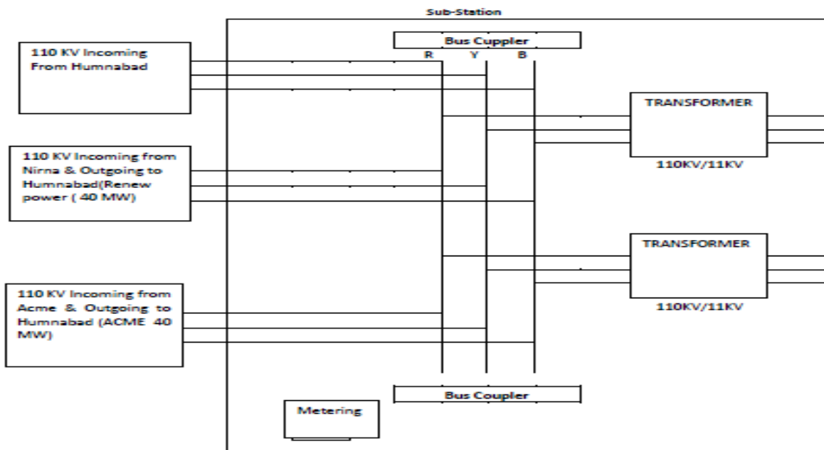
Figure 8 Line diagram of ACME Kaithal Solar Power Private Limited
