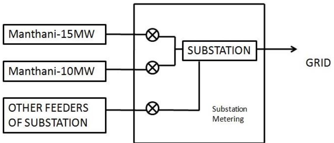
Figure 26 Line diagram of ACME Mahbubnagar Solar 1 (MANTHANI)
