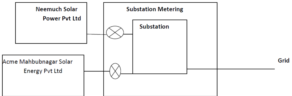
Figure 16 Line diagram of Neemuch Solar Power Pvt. Ltd.
