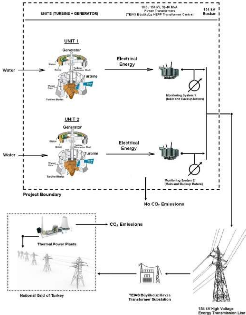
Figure 2. Schematic diagram showing the flow diagram of the project boundary, its connection to national grid, and emission sources and gases included in the project boundary and monitoring variables. The diagram was prepared by the project proponent by using the information given in the turbine specifications brochure 13 , the extended official single line diagram 14 , the simplified official single line
