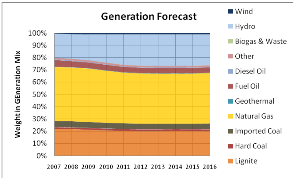
Figure 4. Electricity Generation Forecasts 8
