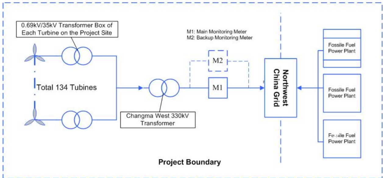
Figure B.3-1 Project Boundary
