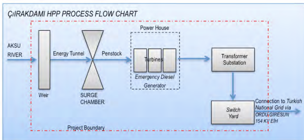
Figure 1: Flow chart showing the basic operational principles of the project activity. The project activity will be connected to the grid via the 154 KV Ordu-Giresun Transmission Line, as indicated in the connection agreement provided to the validating DOE.
