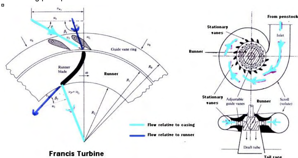
Figure 2: The working principle of a Vertical Axis Francis type turbine.
