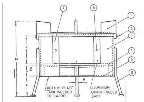
Diagram of Improved Cook Stove
