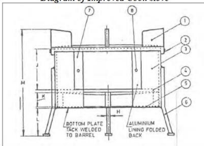
Diagram of Improved Cook stove
