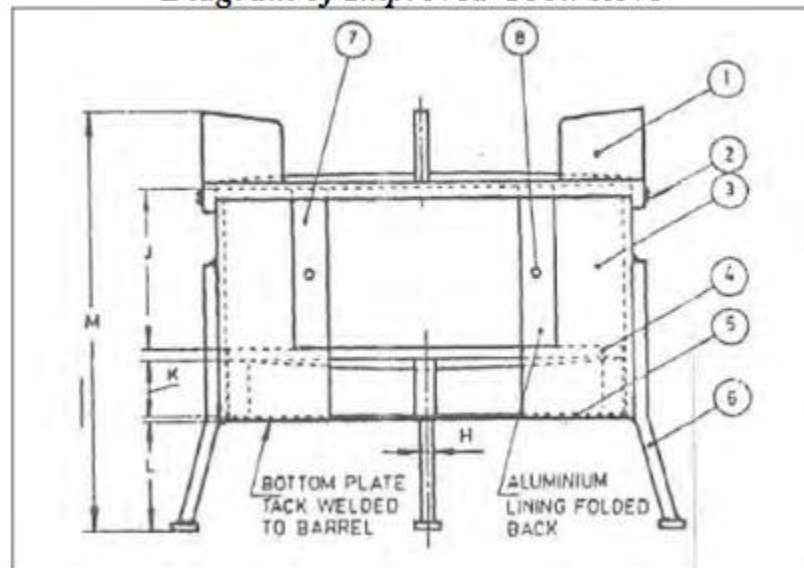
Diagram of Improved Cook stove
