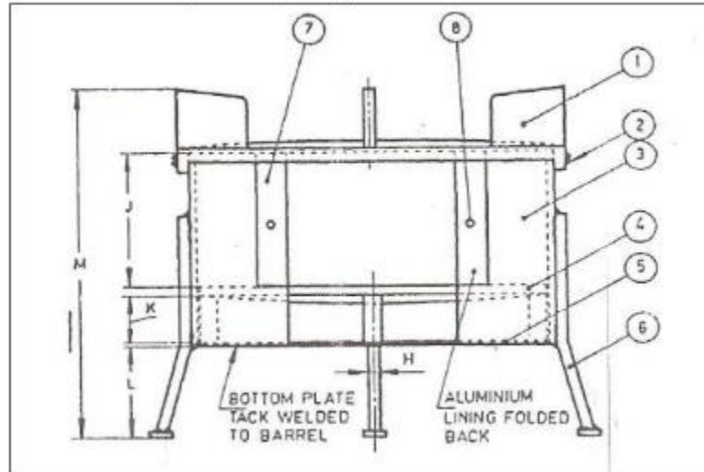
Diagram of Improved Cook stove
