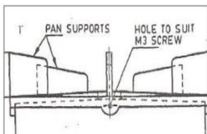
Top Plate
