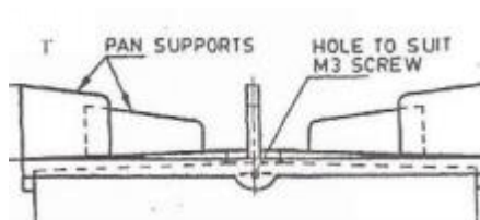
Figure 1.a. Top Plate Figure
