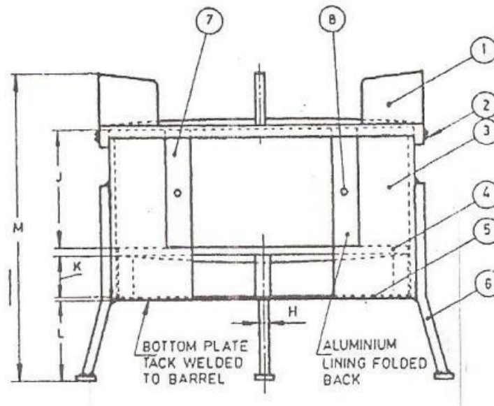
Diagram of Improved Cook stove
