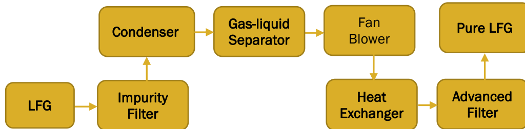
Figure 1.1 The flow chart of the LFG pre-treatment system
