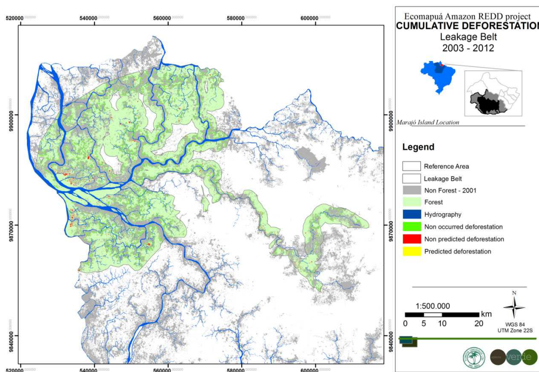
Figure 13. Cumulative deforestation in the Leakage Belt between 2003 and 2012
