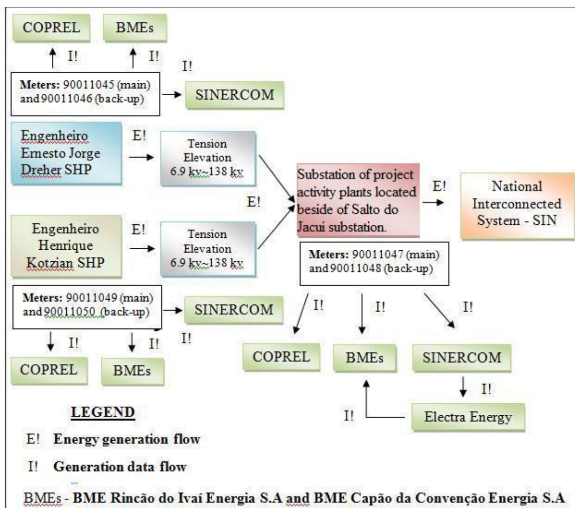
Figure 4: Flow chart of energy and generation data (meters installed can be changed during the project lifetime, so the serial number can be changed also).
