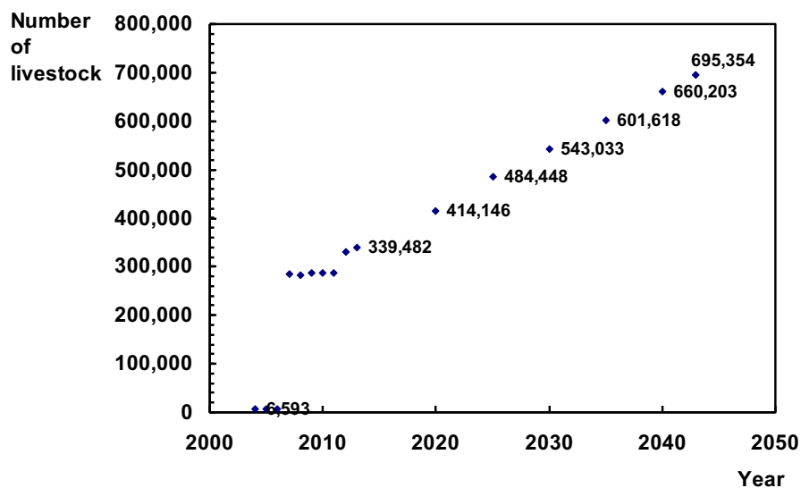
Figure 25. Number of livestock projected to the municipality of Lábrea, State of Amazonas, considering the project duration period (adapted from IBGE, 2014)
