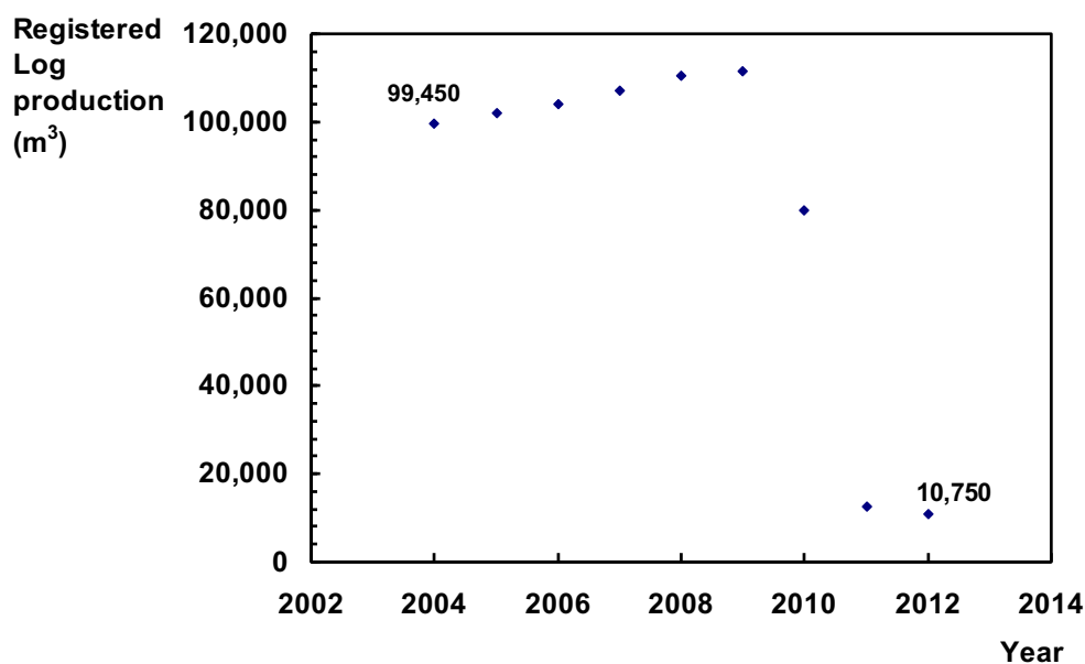
Figure 26. Production of sawmill logs in the municipality of Lábrea, State of Amazonas (IBGE, 2014)
