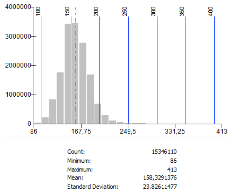
Figure 18. Distribution of altimetry in the Reference Region
