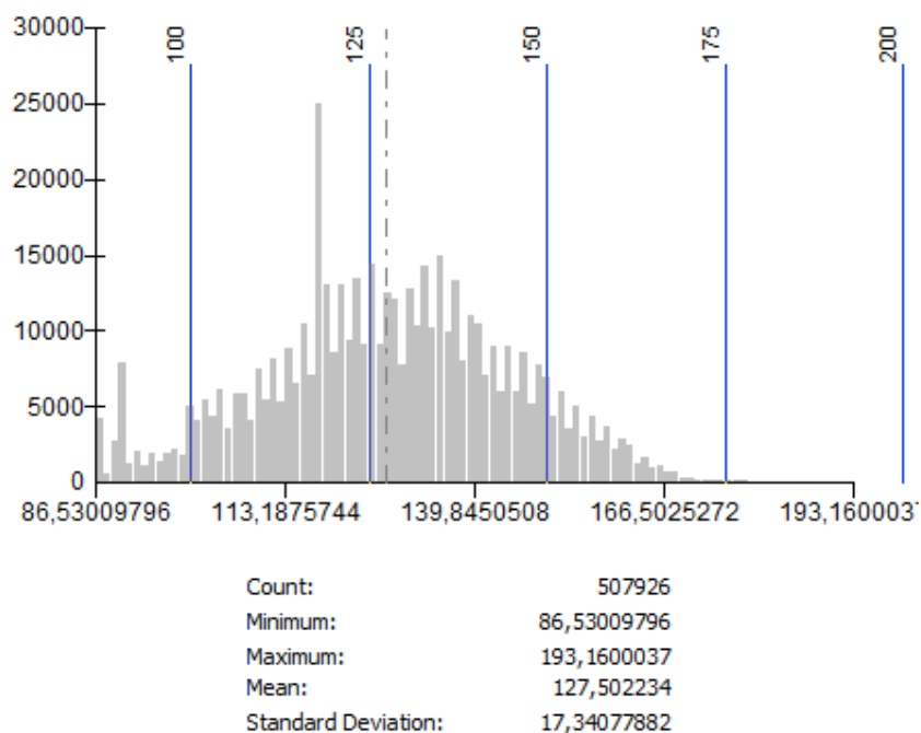
Figure 17. Distribution of altimetry in the Project Area
