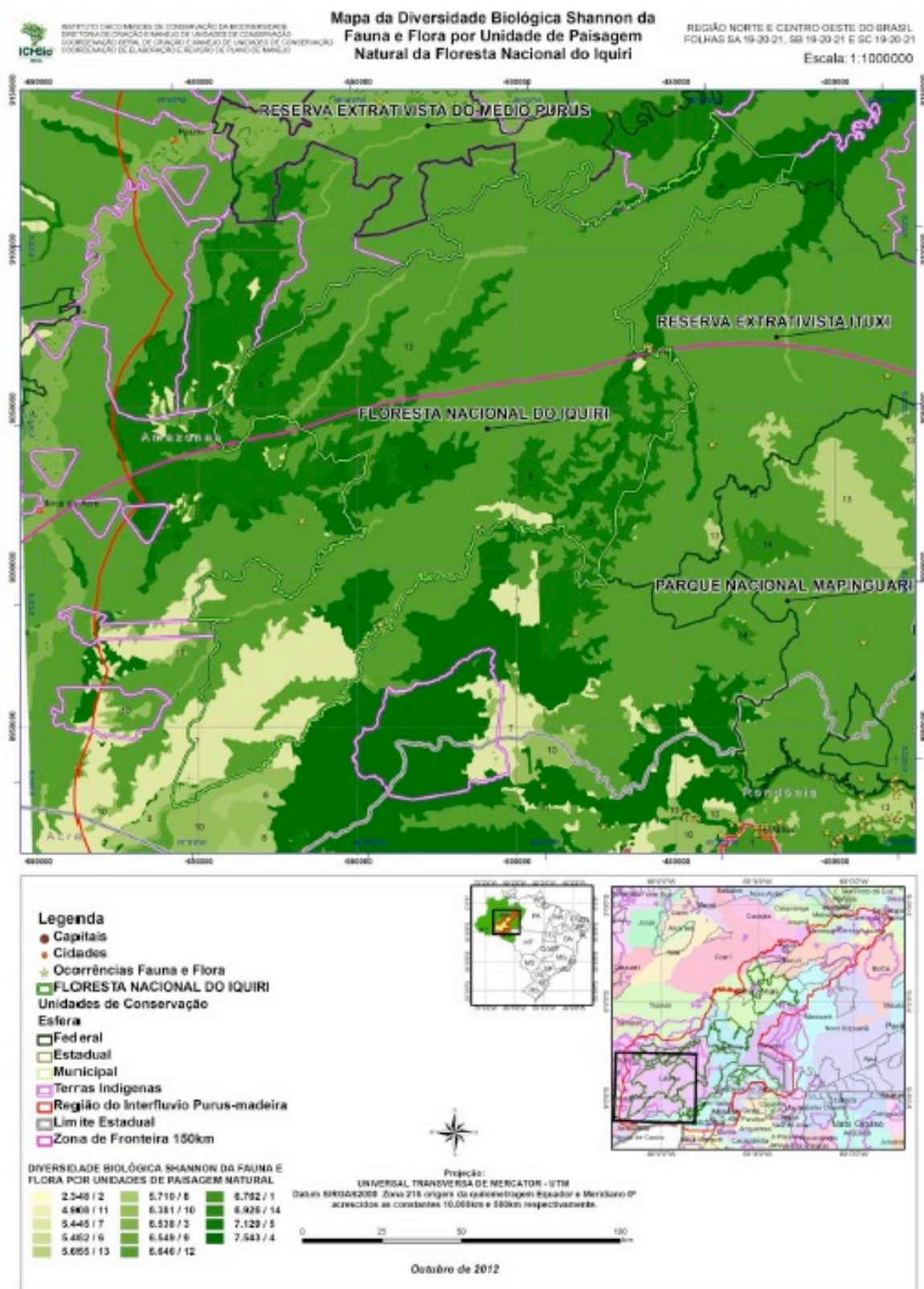
Figure 37. Map of “Shannon biodiversity” in FLONA Iquiri (Fauna and Flora). Source: Irgang (2012)
