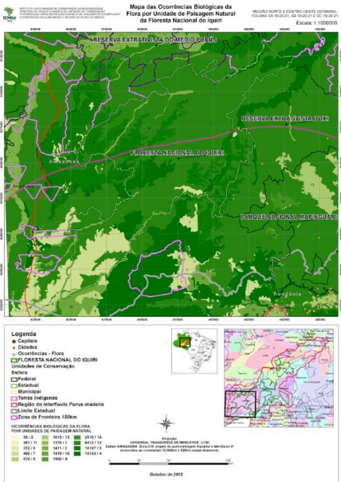
Figure 31. Map of biological occurrences in FLONA Iquiri (Flora). Source: Irgang (2012)
