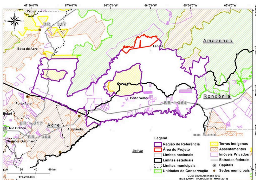
Figure 9. Land use map in the project region, indicating Conservation Units, settlements, indigenous lands (including Kaxarari land) and private lands
