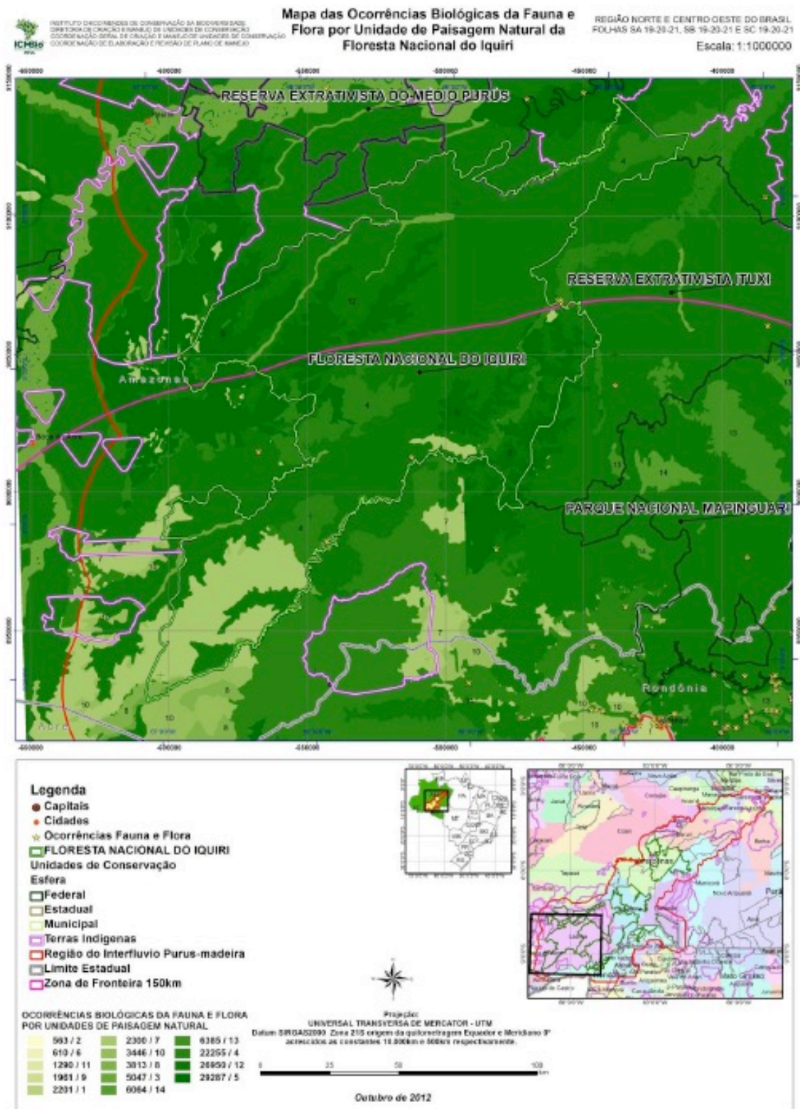
Figure 33. Map of biological occurrences in FLONA Iquiri (Fauna and Flora). Source: Irgang (2012)
