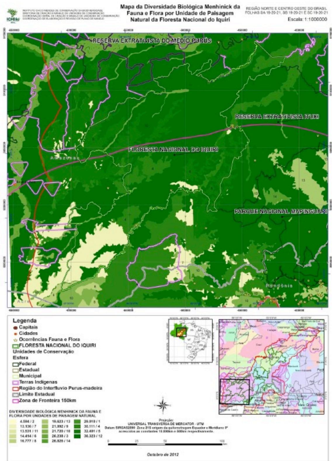
Figure 36. Map of “Menhinick biodiversity” in FLONA Iquiri (Fauna and Flora). Source: Irgang (2012)
