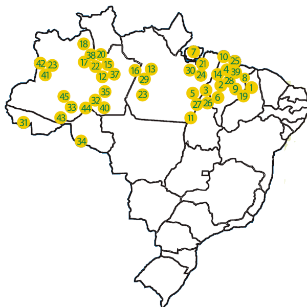
Figure 7. “New Social Cartography of the Amazon”, “Social Movements, Collective Identity and Conflicts”: 33 - “Extractive Communities of the Resex Ituxi”; 43 - “Indigenous peoples of the municipality of Lábrea”
