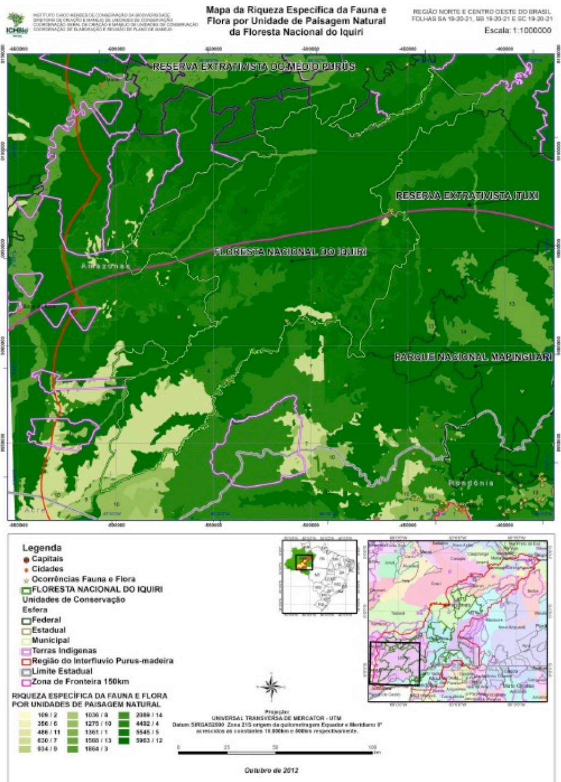
Figure 34. Map of specific richness in FLONA Iquiri (Fauna and Flora). Source: Irgang (2012)
