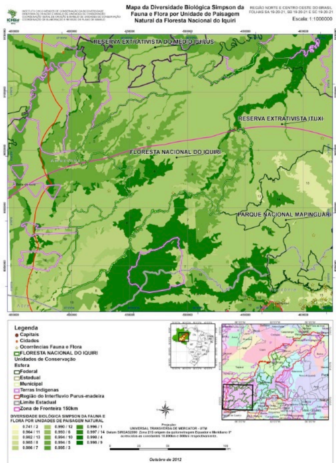
Figure 38. Map of “Simpson biodiversity” in FLONA Iquiri (Fauna and Flora). Source: Irgang (2012)
