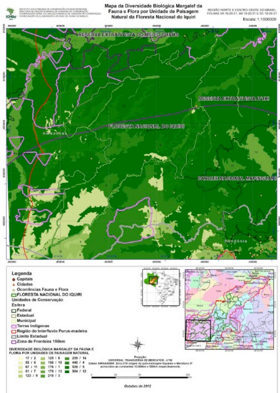
Figure 35. Map of “Margalef biodiversity” in FLONA Iquiri (Fauna and Flora). Source: Irgang (2012)
