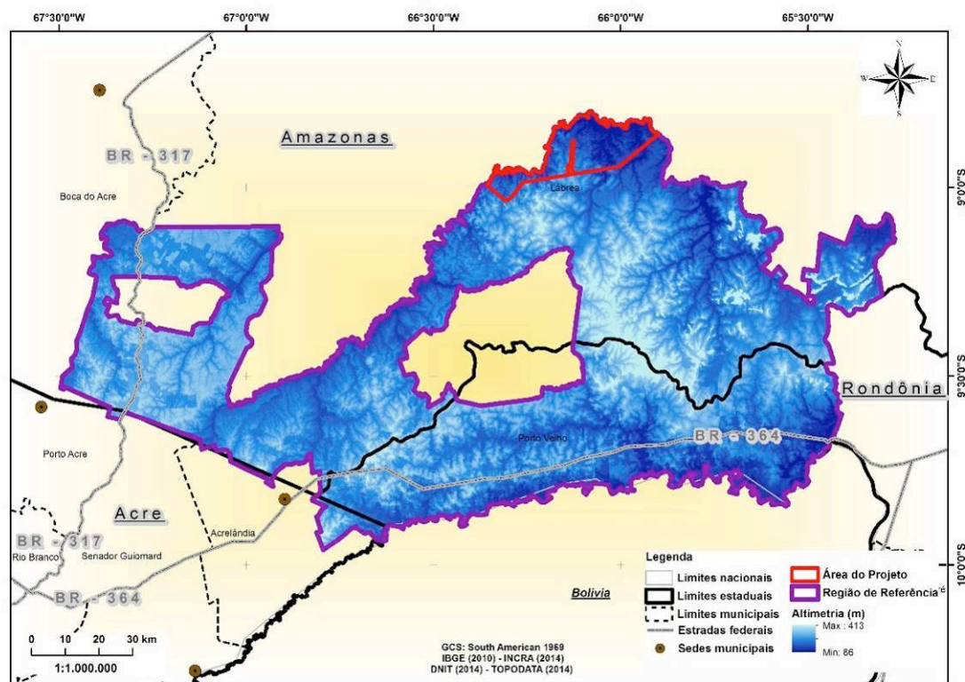
Figure 16. Altimetry characterization for the Reference Region and Project Area
