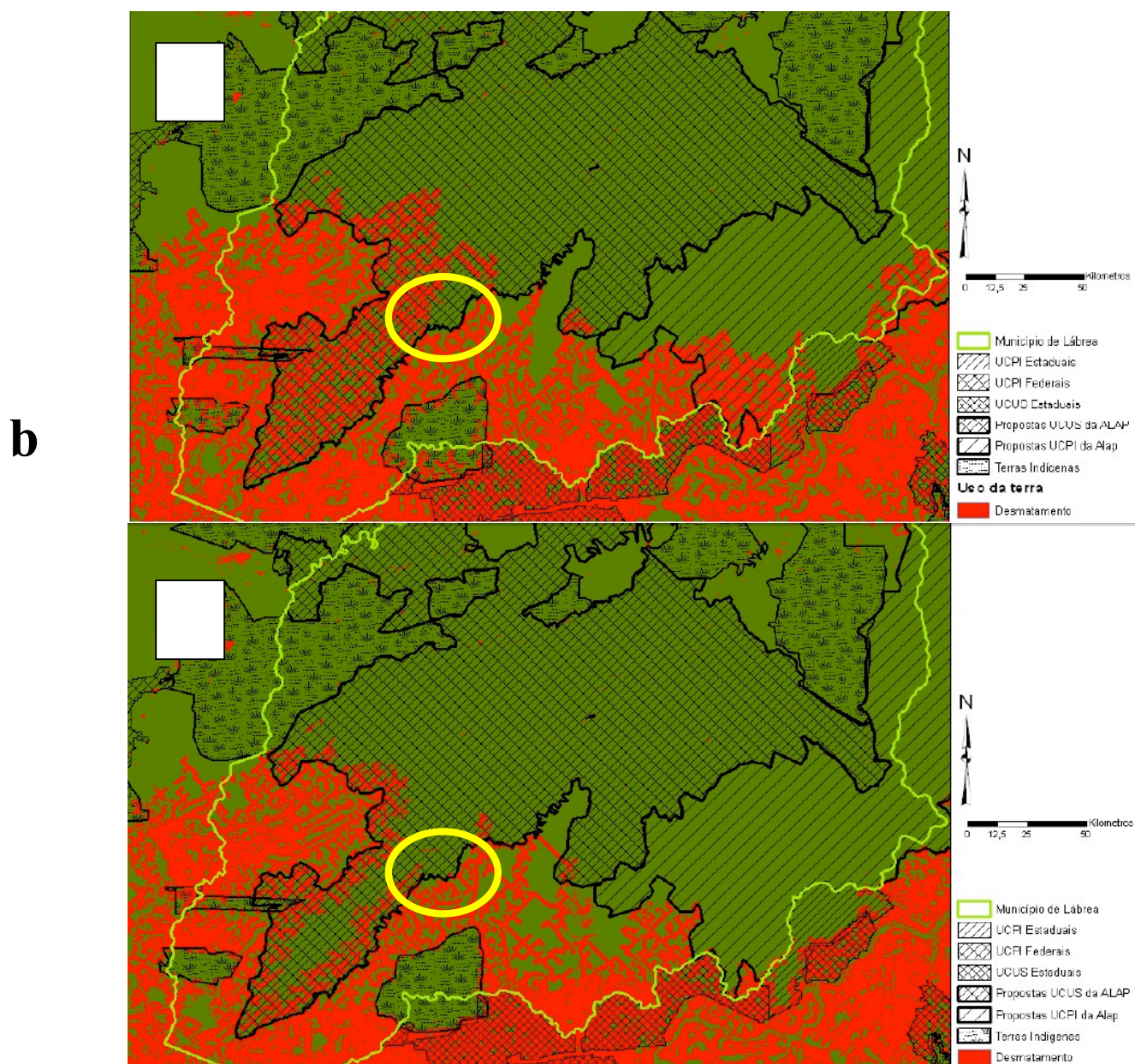
Figure 4. Maps of land cover representing deforestation in the municipality of Lábrea in 2040. a. Scenario not considering the recently-created conservation areas. b. Scenario considering the recently-created conservation areas (Source: VITEL, 2009).
