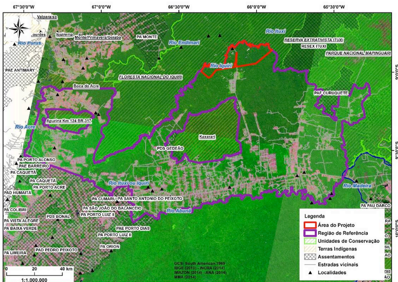
Figure 13. Location of the Reference Region and Project Area
