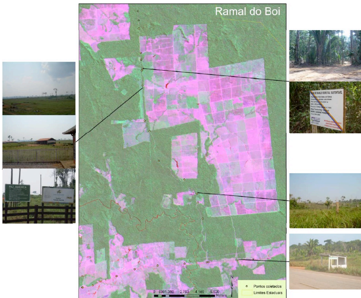
Figure 3. Region of “Ramal do Boi” (road) visited in August 2008, with photographs taken in the field representing the main land uses: cattle ranching and forest management. The same land-use pattern was reported to “Ramal do Jequitibá” (Source: VITEL, 2009).
