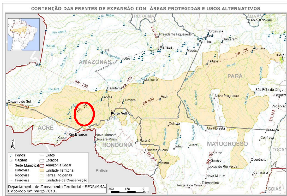
Figure 11. Containment of the expansion fronts with protected areas and alternative uses (Source: Brazilian Ministry of Environment)
