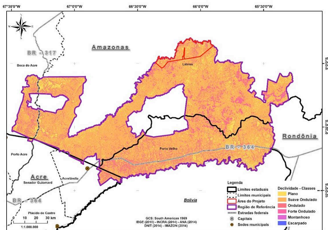
Figure 19. Characterization of landscape relief in the Reference Region and Project Area
