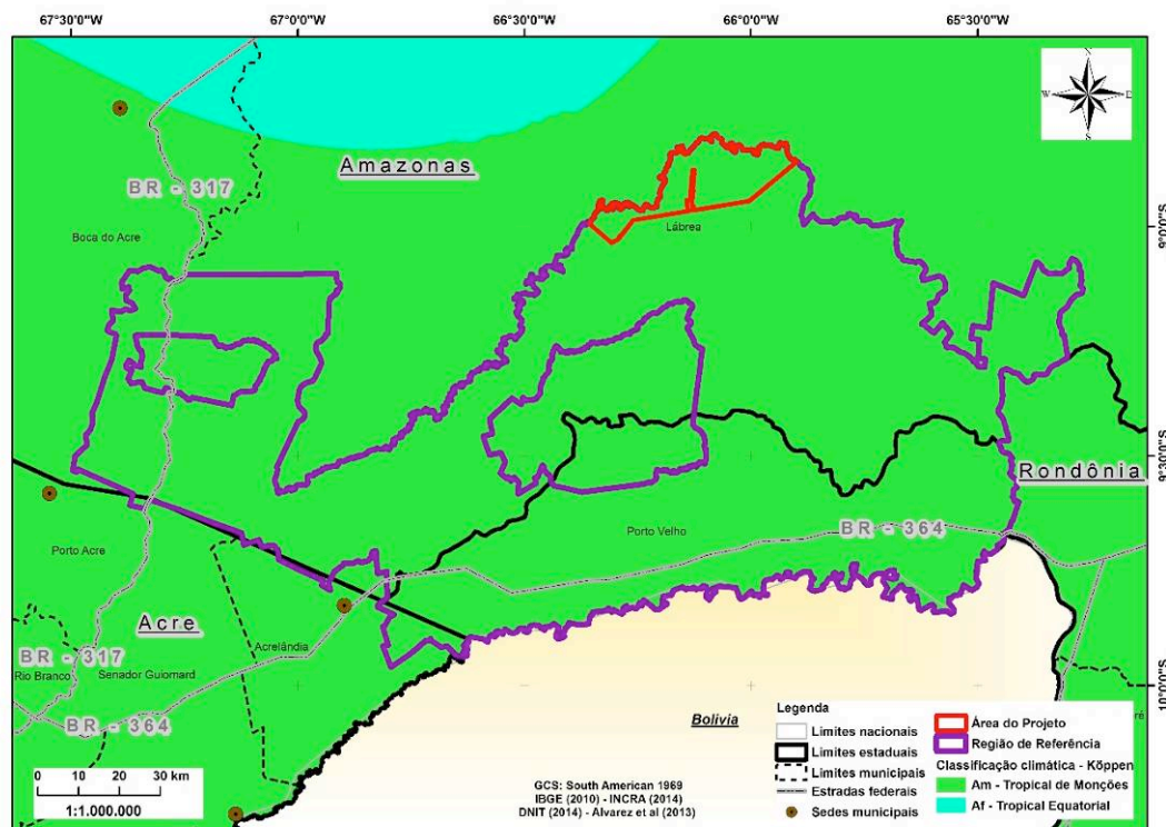
Figure 21. Characterization of climate in the Reference Region and Project Area
