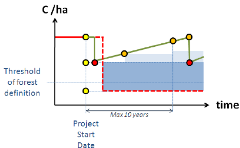
Figure 12. Carbon balance in project category B of VM0015 methodology
