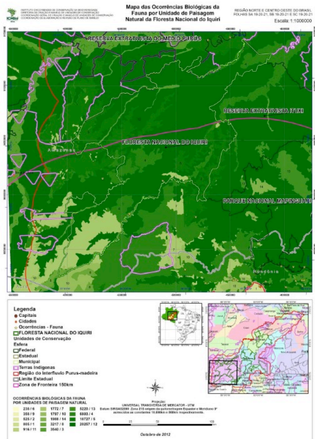
Figure 32. Map of biological occurrences in FLONA Iquiri (Fauna). Source: Irgang (2012)
