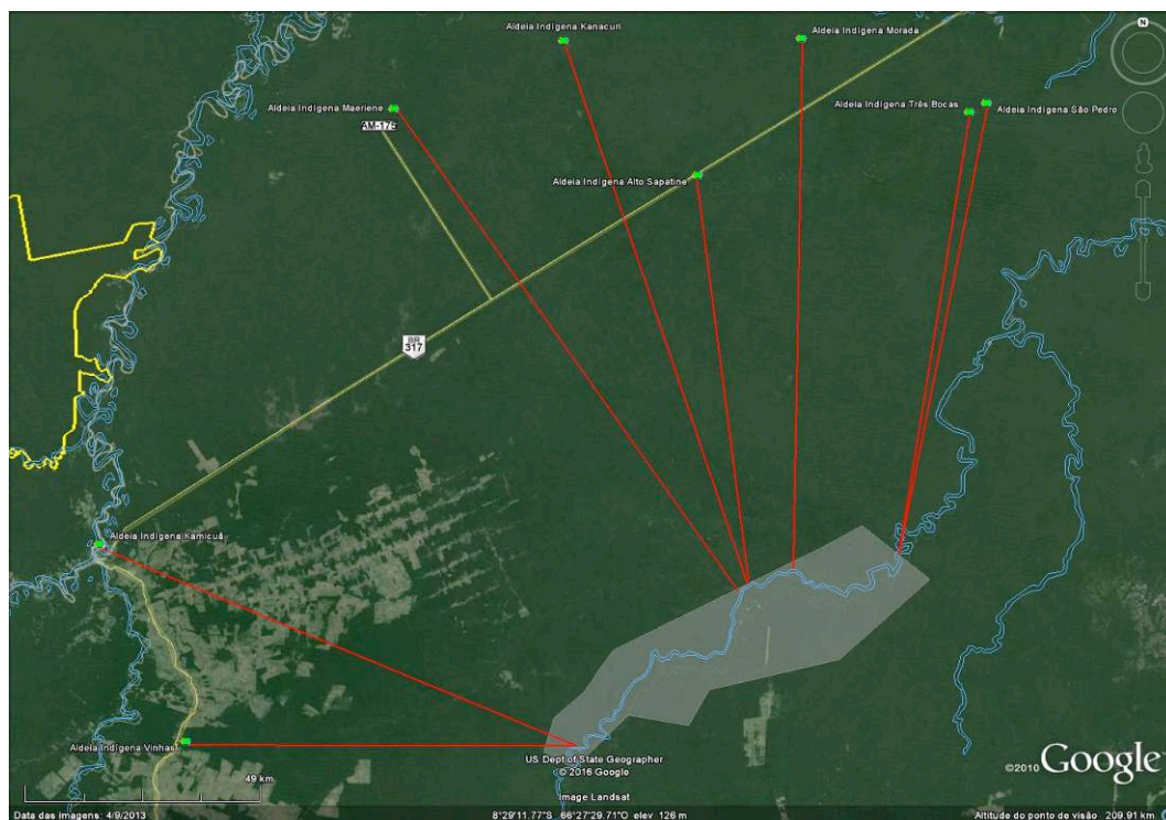
Figure 8. Location of indigenous villages in the project region
