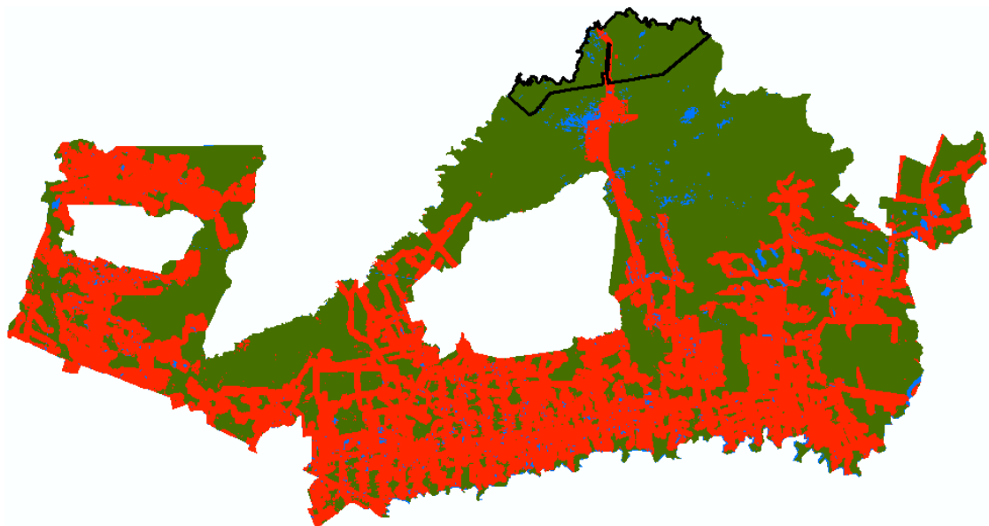
Figure 27. Mapping of cumulative deforestation projected to 2043, for the Reference Region
