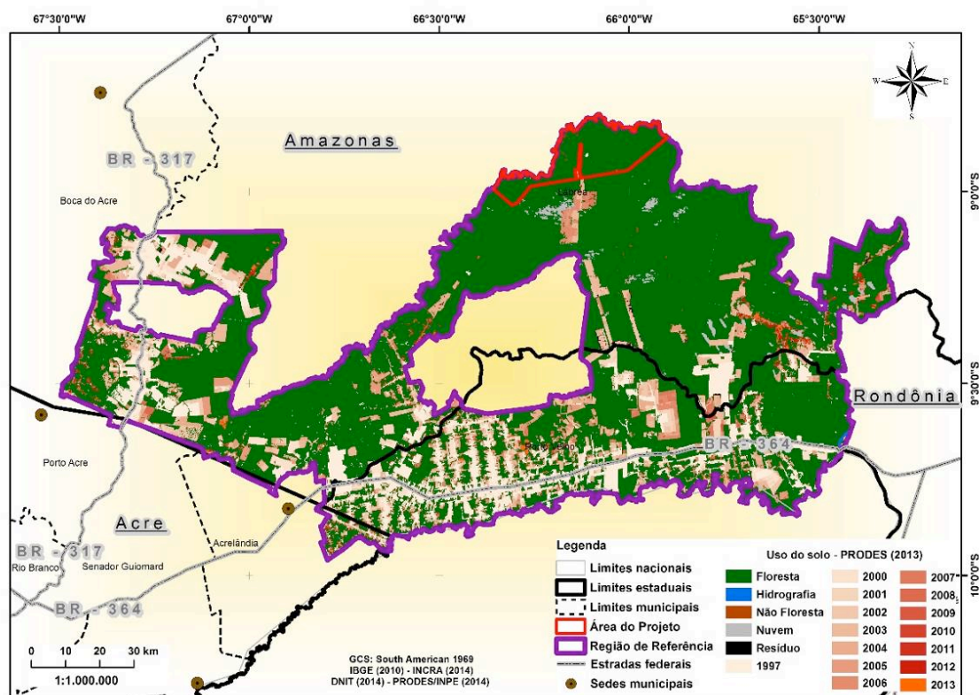
Figure 23. Mapping of land use in 2013, for the Reference Region and Project Area. Source: PRODES Digital (2013)
