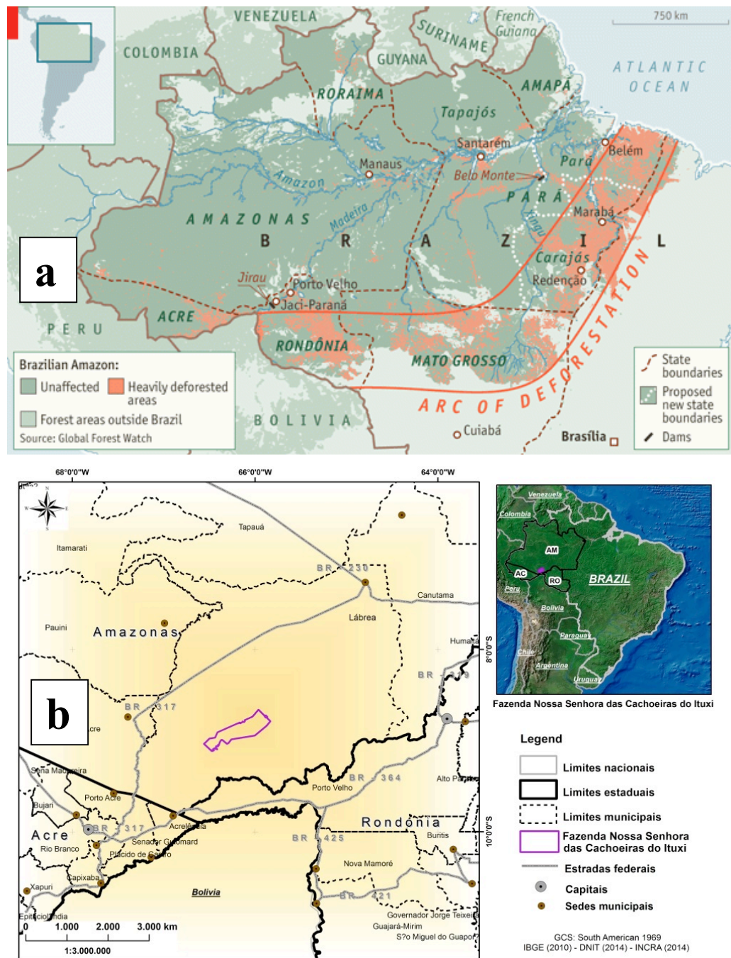
Figure 1. a. Location of the “Arc of Deforestation”. Source: The Economist (2011) 2 . b. Overview of the location of FORTALEZA ITUXI REDD PROJECT. The main deforestation risks are located from the western and southern regions of the Project Area.
