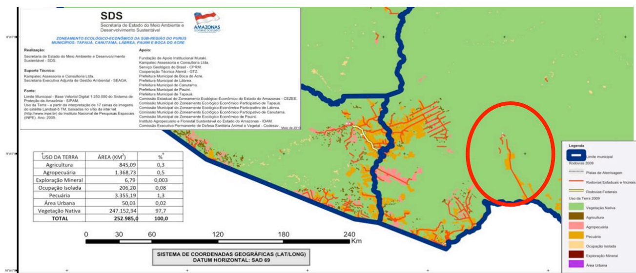
Figure 5. Map of land use in the project region in 2009, showing predominance of pasture as final land use in deforested areas (Source: MMA, 2009).
