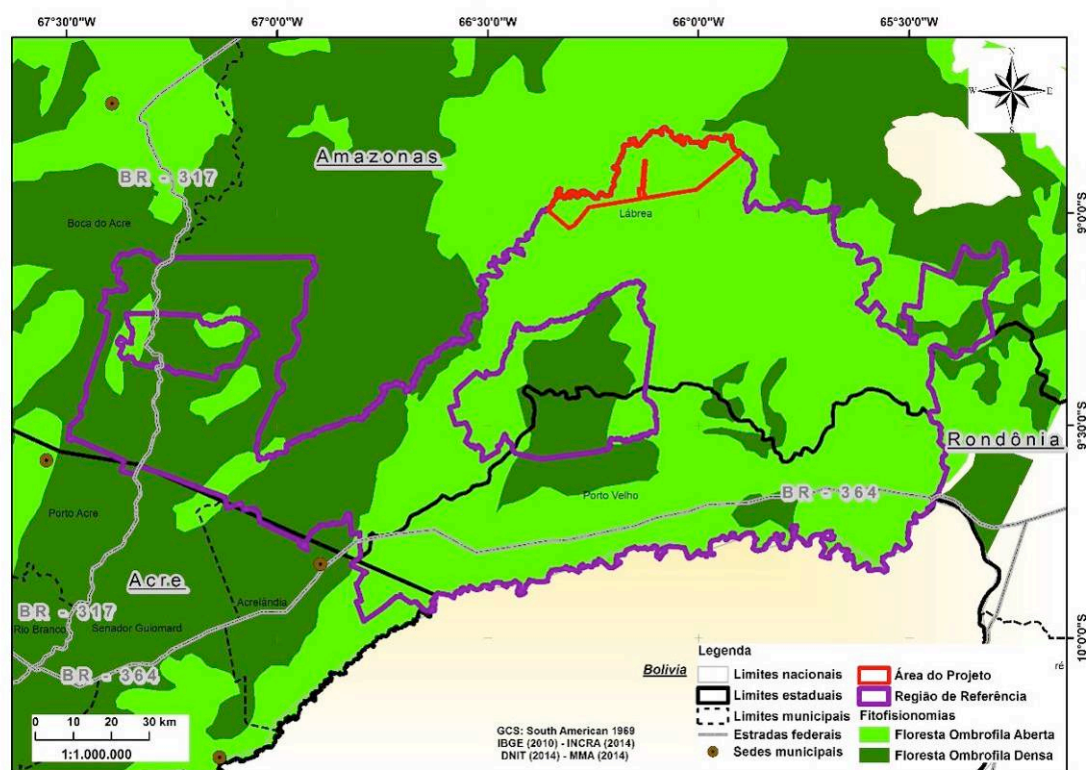
Figure 15. Characterization of forest typologies in the Reference Region and Project Area
