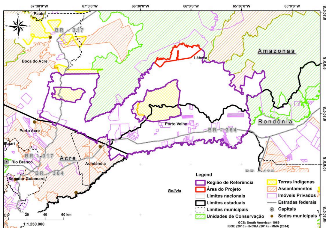
Figure 14. Characterization of land occupation in the Reference Region and Project Area
