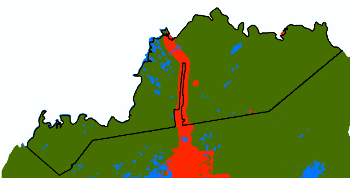
Figure 28. Mapping of cumulative deforestation projected to 2043, for the Project Area
