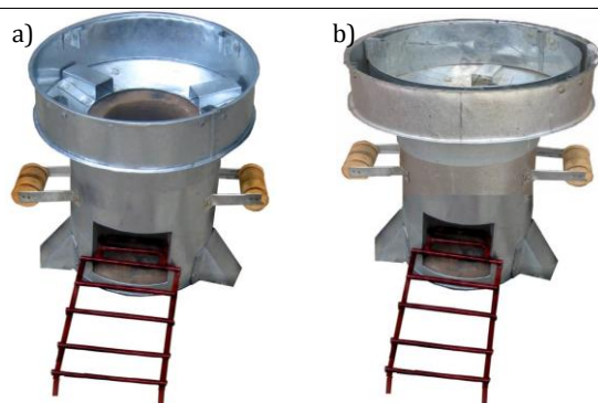
Figure 5: (a) Single and (b) double skirt Tikikil stove models 8
