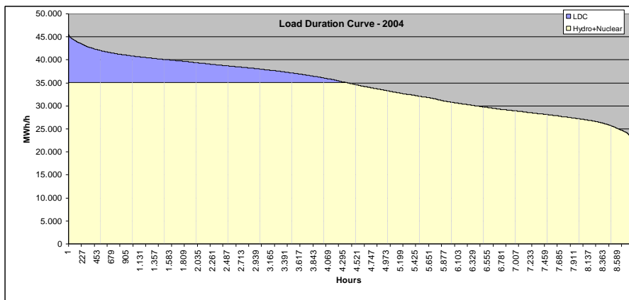
Figure 8. Load duration curve for the S-SE-CO system, 2004
