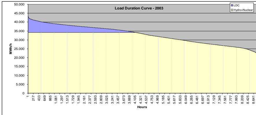
Figure 7. Load duration curve for the S-SE-CO system, 2003
