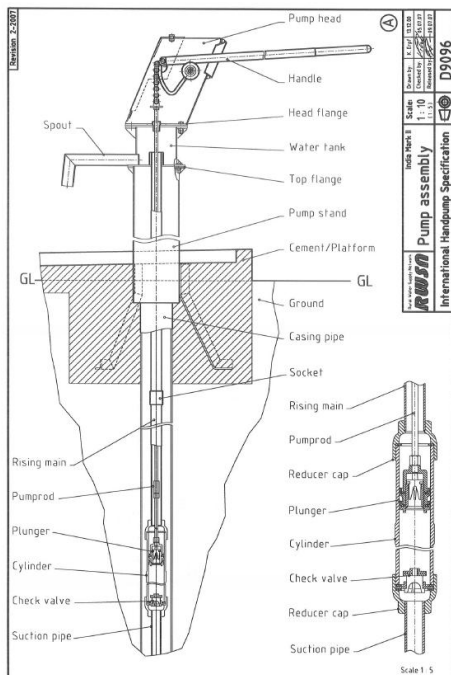
Figure 3: Diagram and specifications of India Mark II hand pump.
