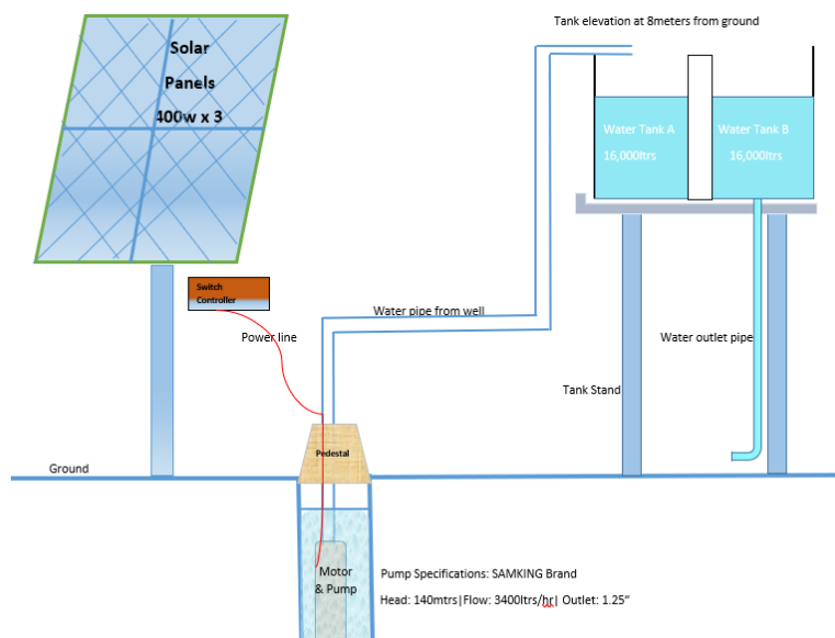
Figure 4: A line diagram of the specification of the solar borehole technology for the Omoro Solar Pump (LAN086).
