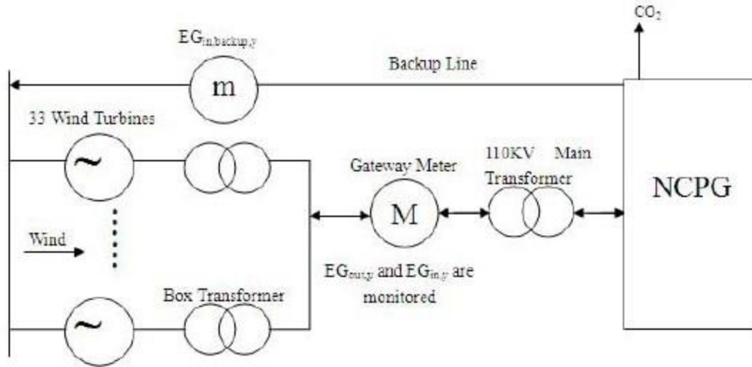
Figure 2. Monitoring points
