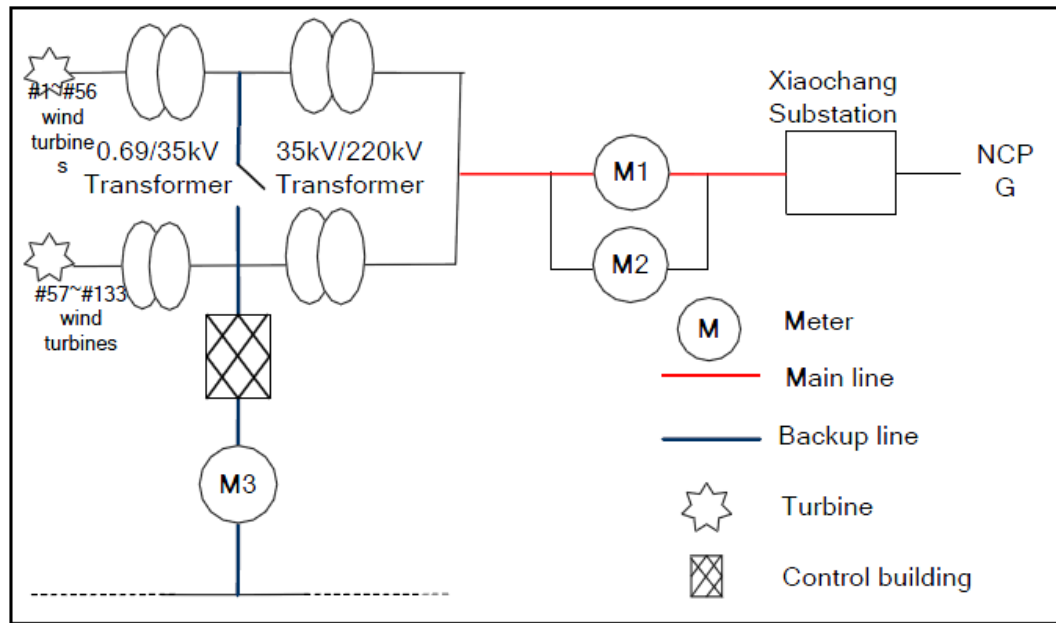
Figure 3 Simplified electrical grid connection diagram
