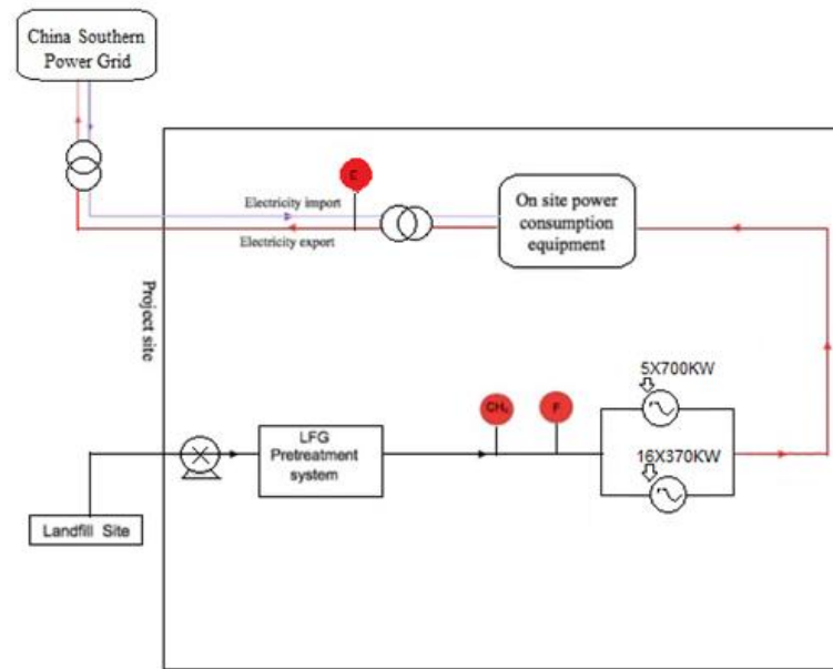
Figure 5.2 The monitoring flow chart
