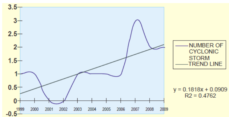
Figure 5 Frequency of cyclone storm over Northern Bay of Bengal (WWF 2010)
