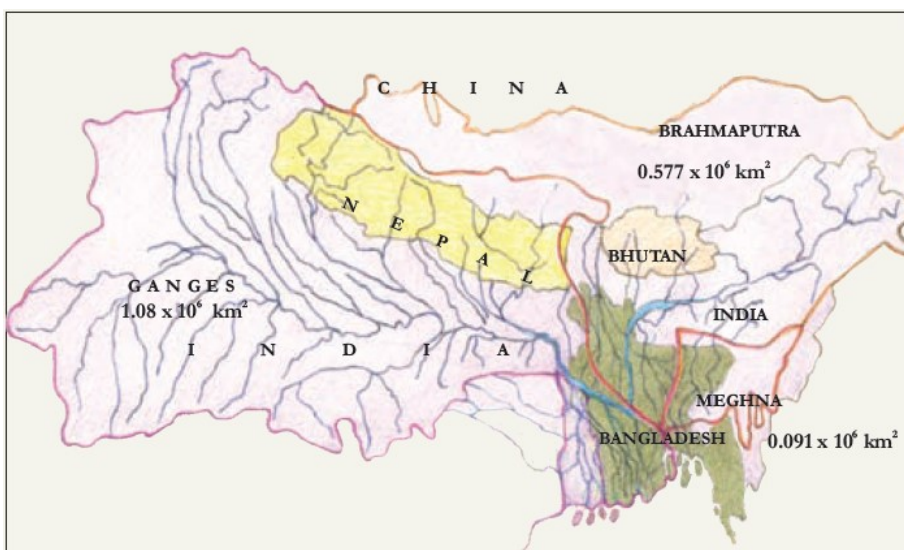
Figure 7 The Ganges-Brahmaputra-Megha system
