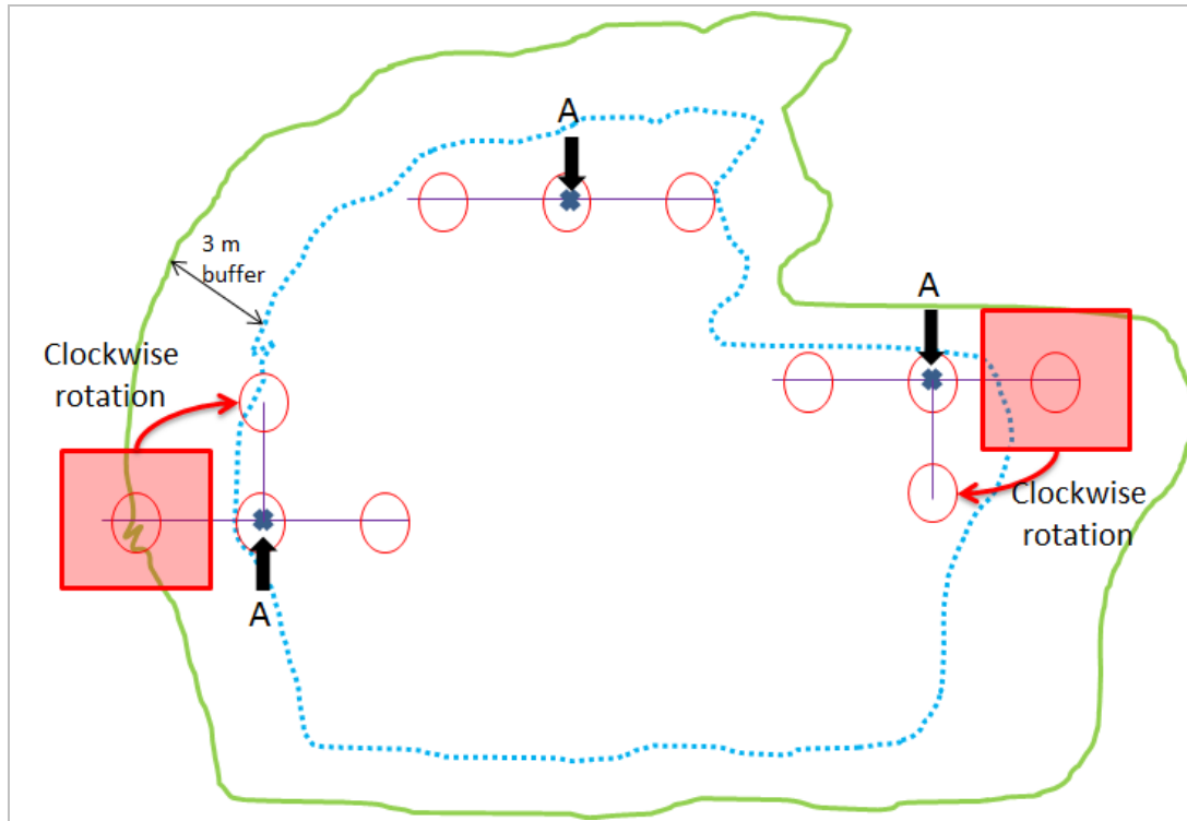
Figure 7 Different conditions of sample plot layouts in the field
