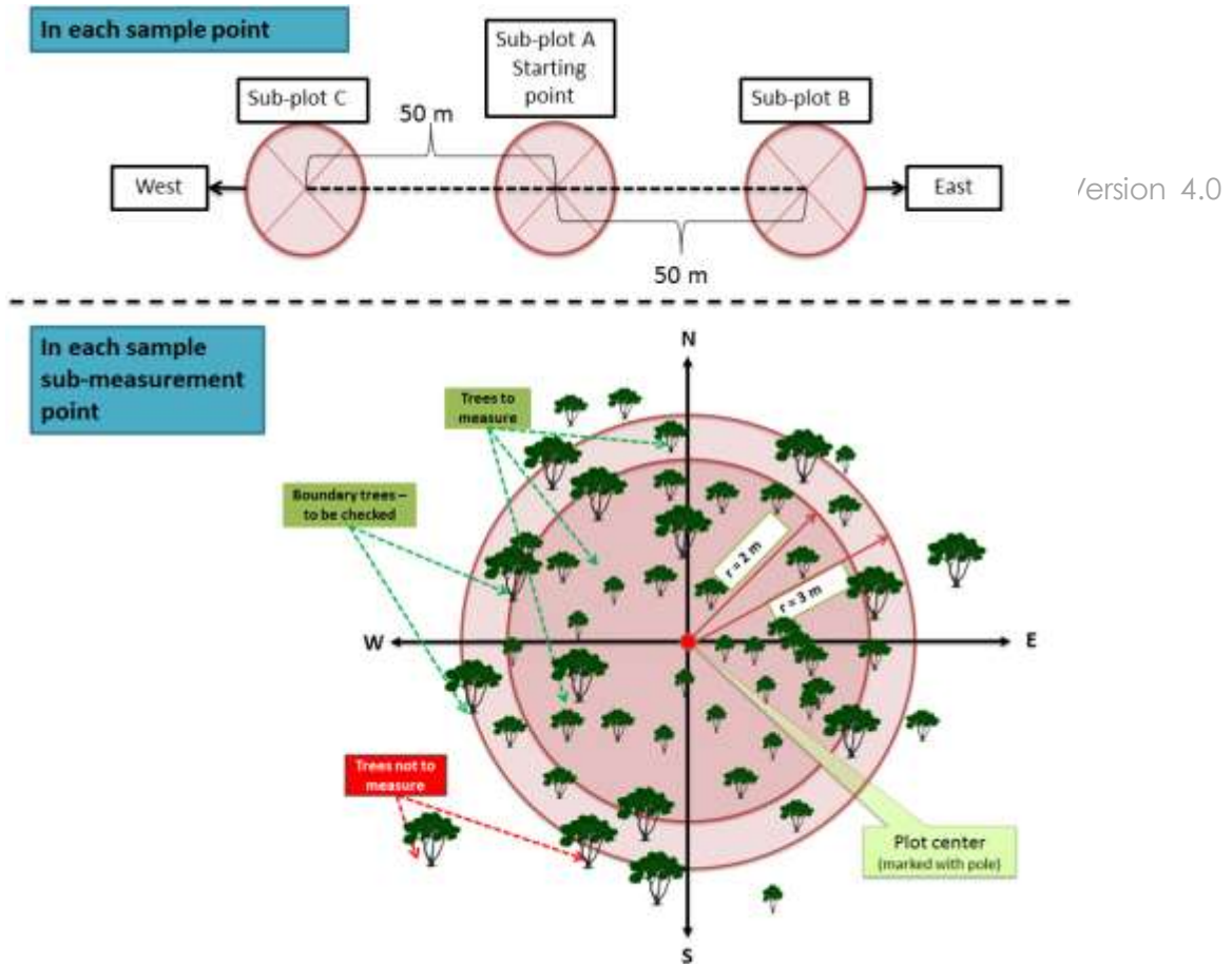
Figure 7 NEWS Carbon inventory plot layout
