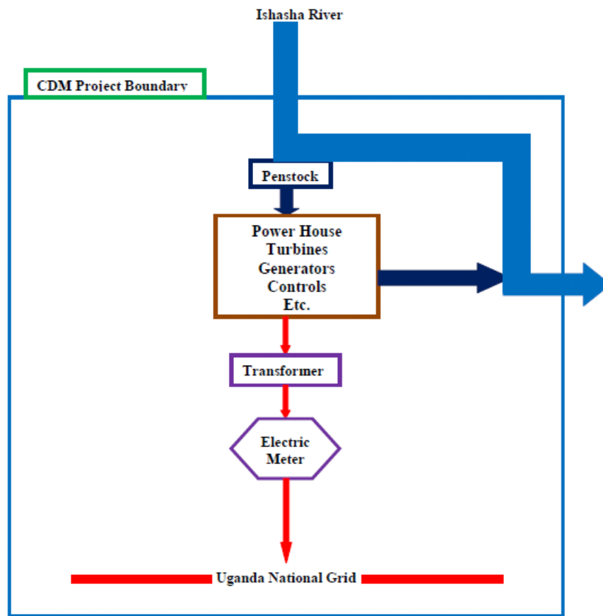
Figure 3: Flow Diagram of Ishasha 6.6 MW Small Hydropower Project
