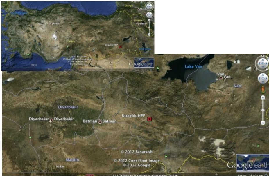
Figure 3:Map showing the location of Kirazlık HPP (red dot within the inset map) on the Botan River,Siirt,Turkey
