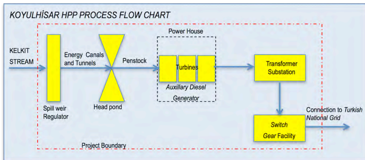
Figure 1: Flow chart showing the basic operational principles of the project activity.
