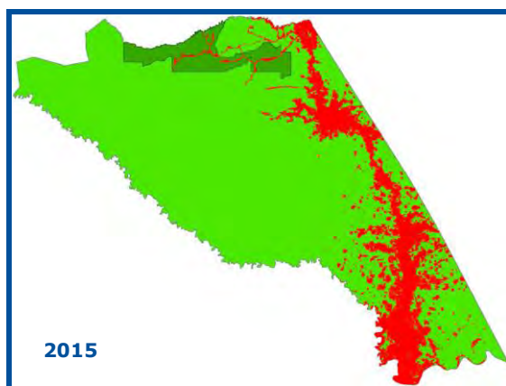
Fig. 84: Deforestation map interpreted up to 2015 (projected and modeled)
