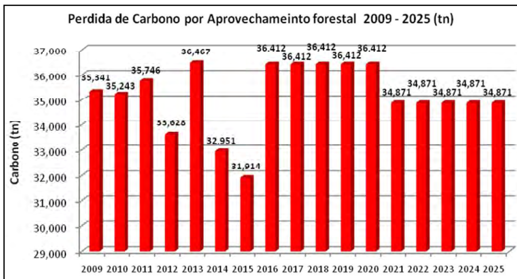
Graph 26: Projected carbon loss due to wood extraction (2009-2025)
