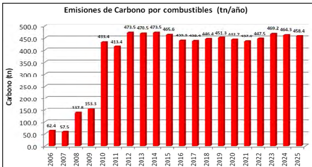
Graph 24: Emissions due to the use of fuels
