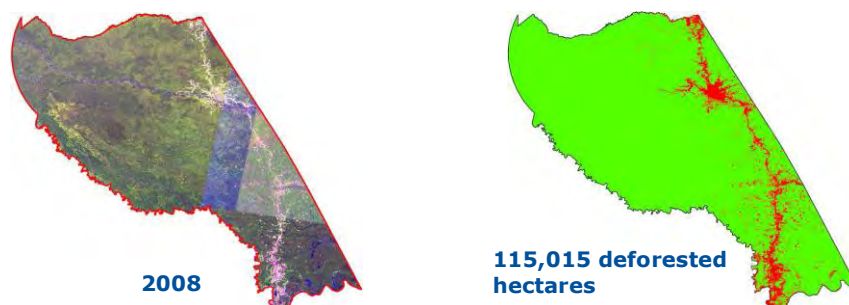
Fig. 73: Quantification of the deforestation using Landsat image 2008
