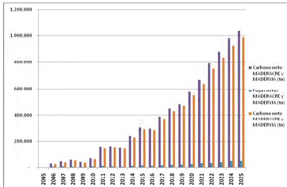
Graph 38: Total net carbon flow for the Madre de Dios Amazon REDD Project
