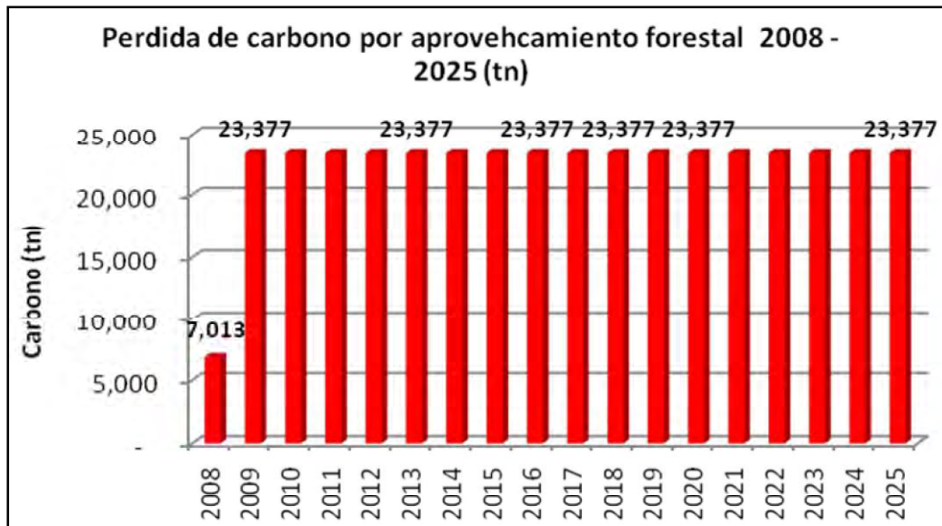
Graph 33: Carbon loss due to wood extraction (2008-2025)
