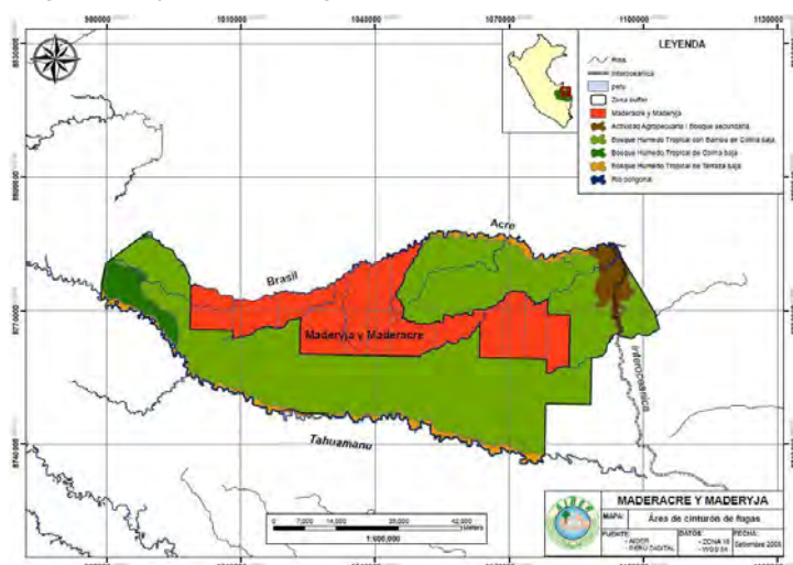
Fig. 67: Map of the leakage belt area
