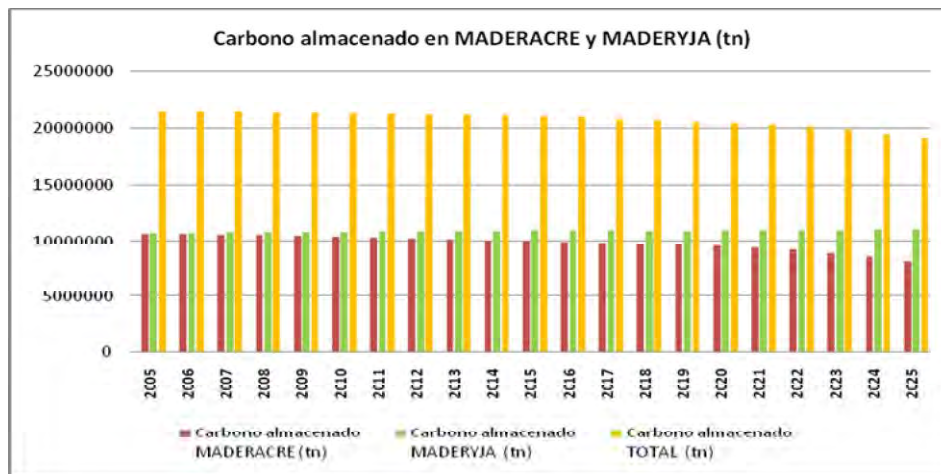
Graph 23: Carbon stocked within the Maderacre and Maderija concessions forests
