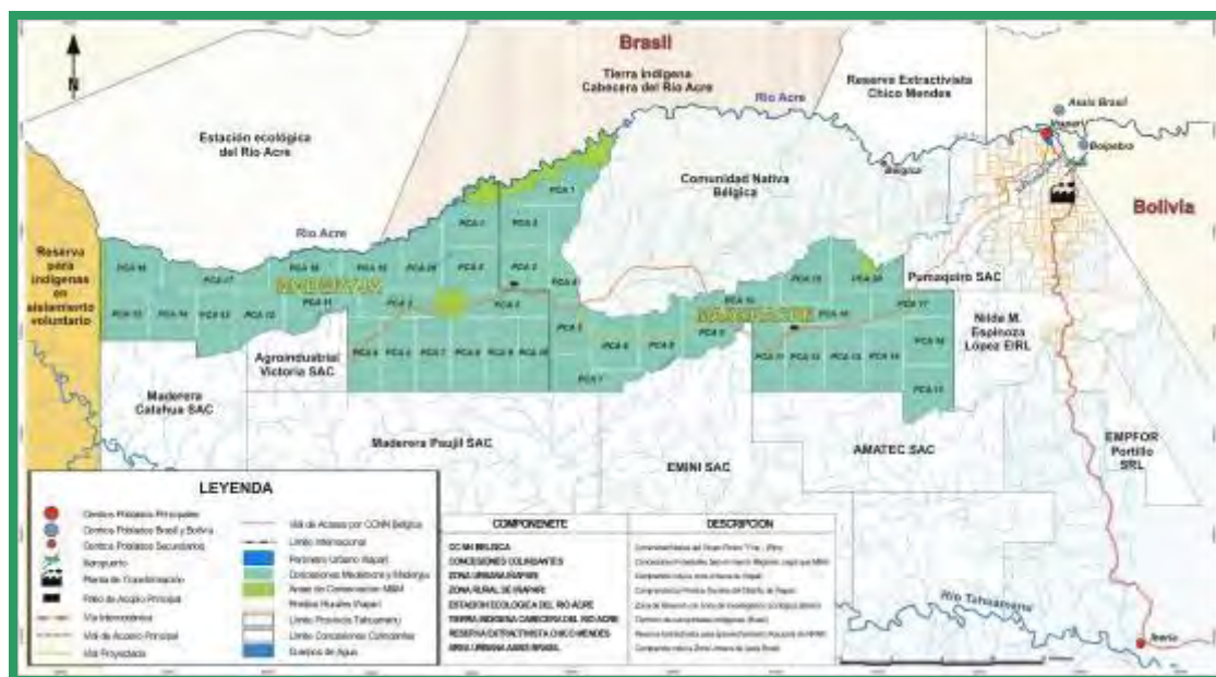
Fig. 64: Map showing the closeness between the concessions and the IIRSA road
