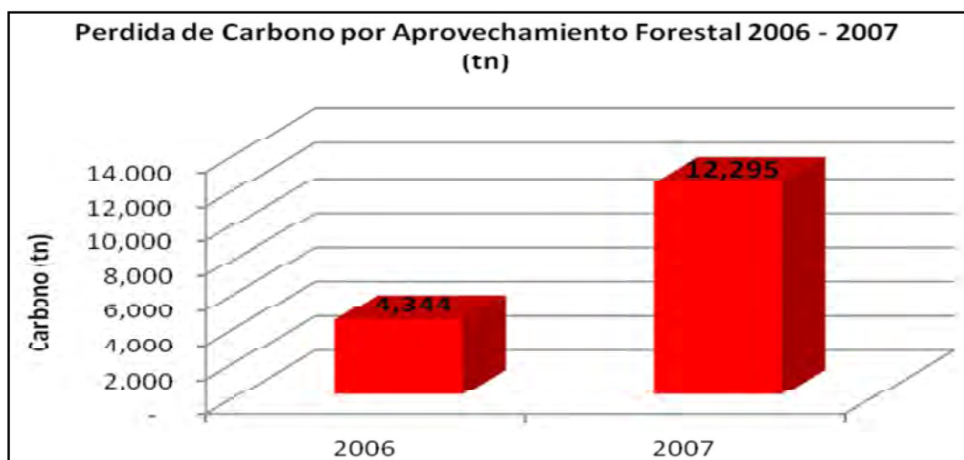
Graph 32: Carbon loss due to wood extraction (2006-2007)
