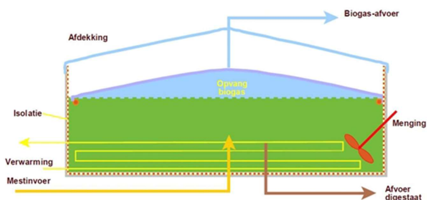
Figure 2: Manure digester operation principle
