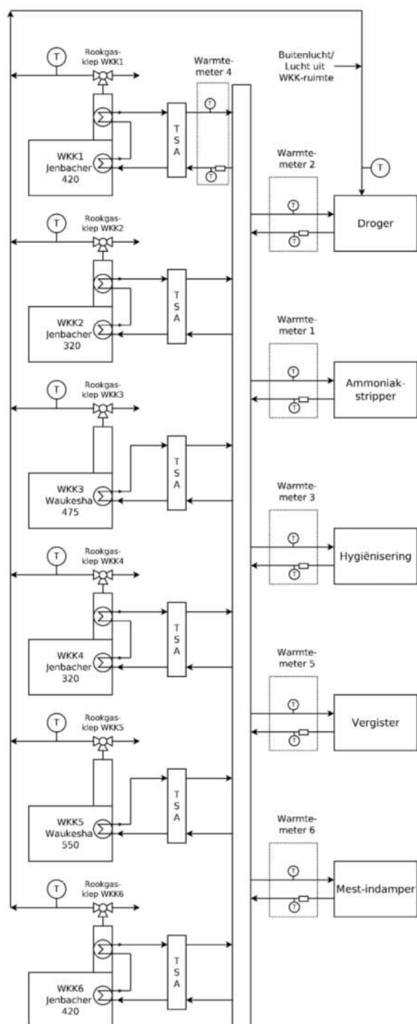
Figure 9: schematic representation of heat utilization 42
