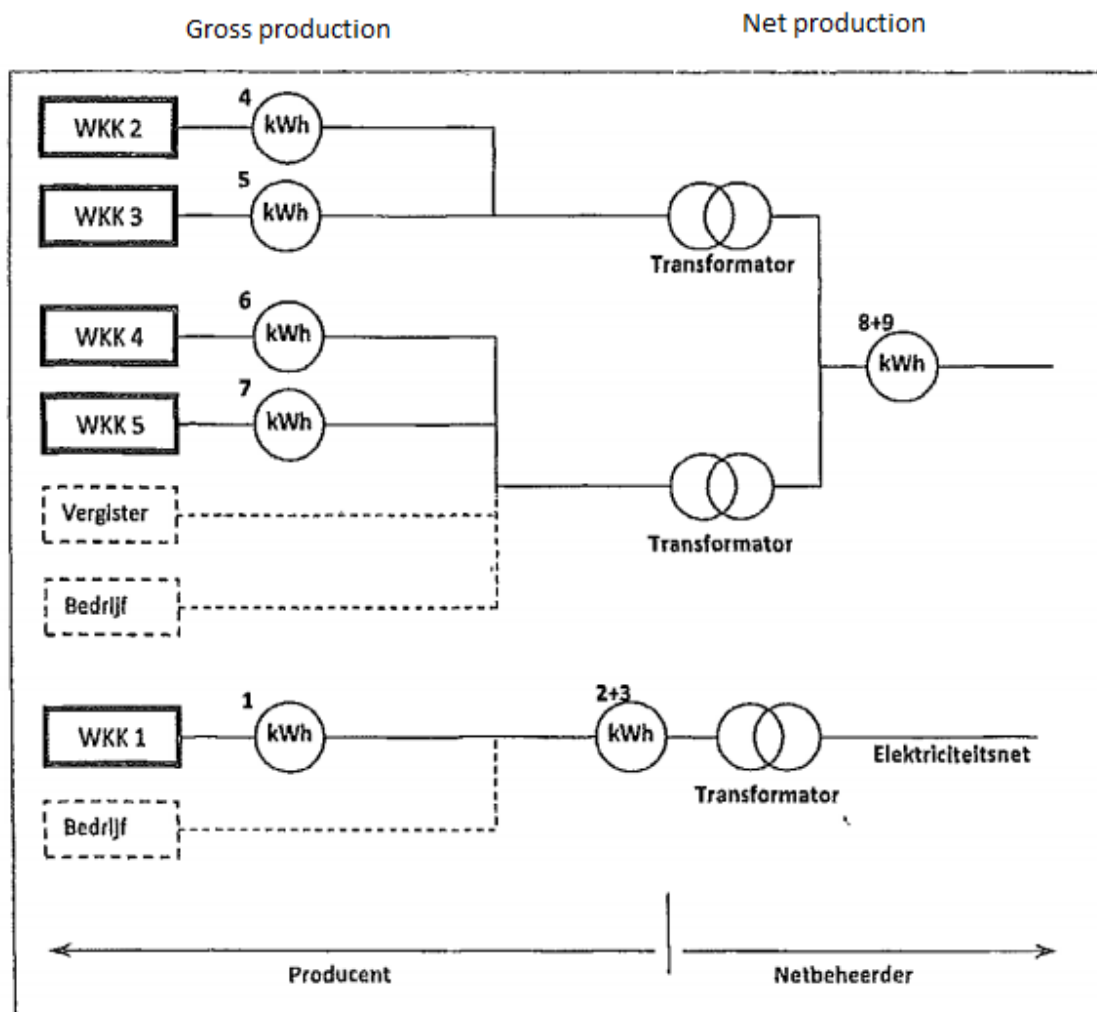
Figure 1 : Schematic representation of electricity flows including system limit and meters (Source: “Meetprotocol elektriciteit en warmte - Princepeel - 2012”, p. 9)
