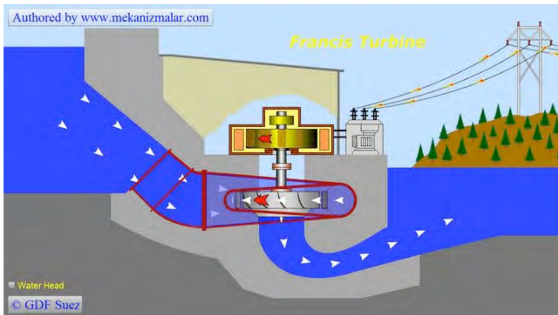
Figure 2: The working principle of a Francis type turbine.
