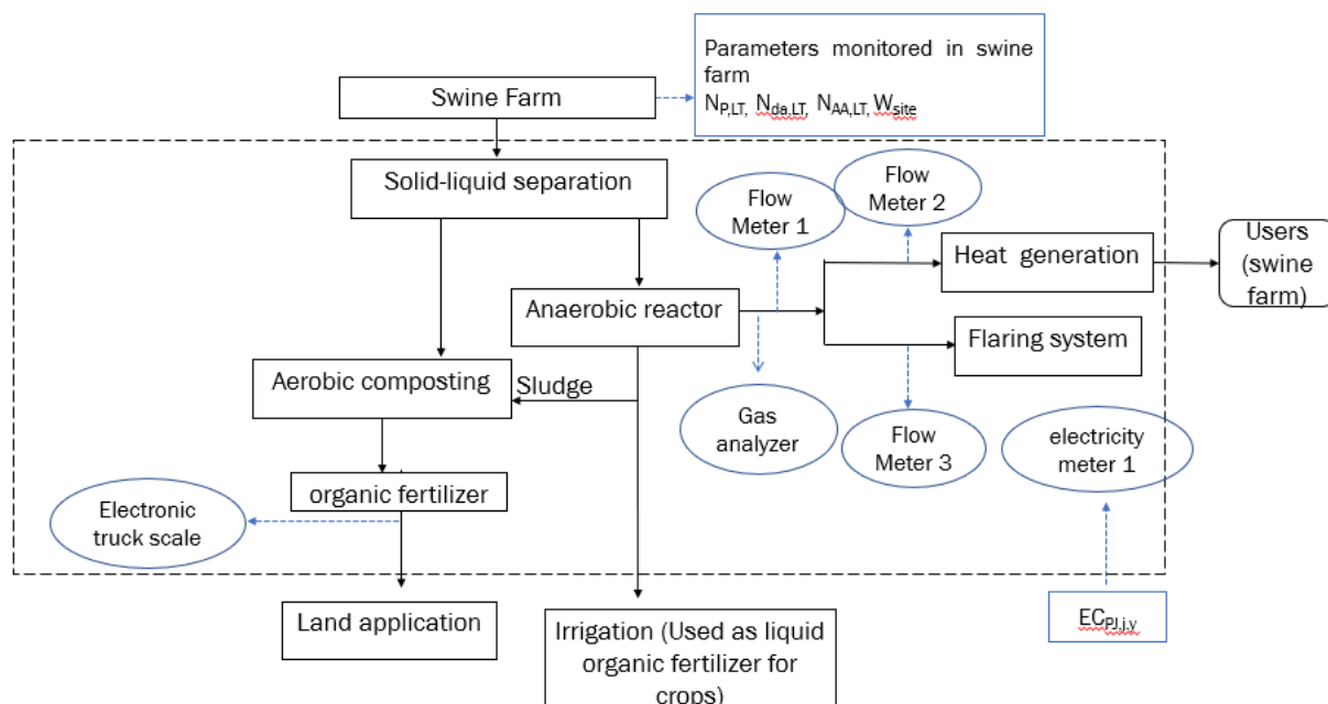
Figure 5-2 Installation and Configuration of Meters
