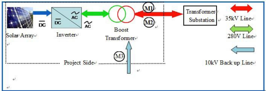
Figure 3 : Power Connection Diagram
