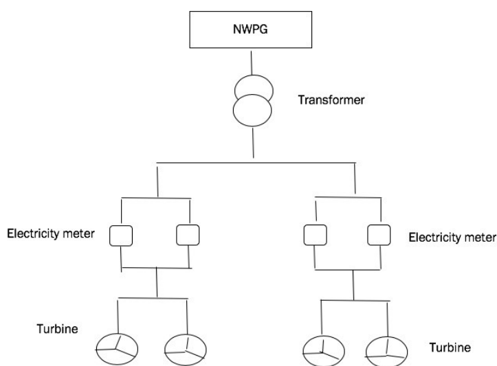
Figure 3. Line Diagram
