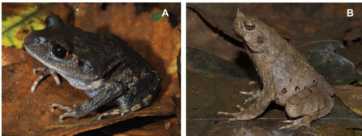
Figure 5.5 Two new species of frogs discovered within the Project Area: (A) Mouhot's litter frog, and (B) O'Reang horned frog
