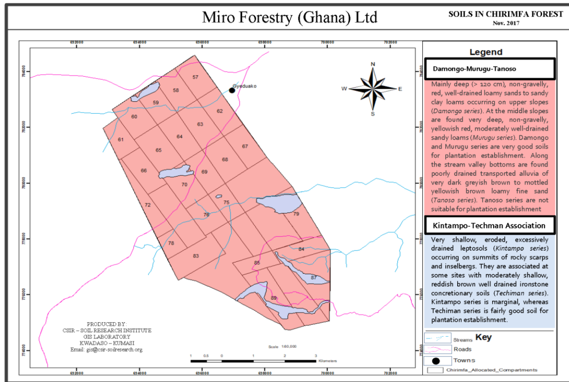
Figure 11. Soil map of selected compartments in the Chirimfa Forest Reserve
