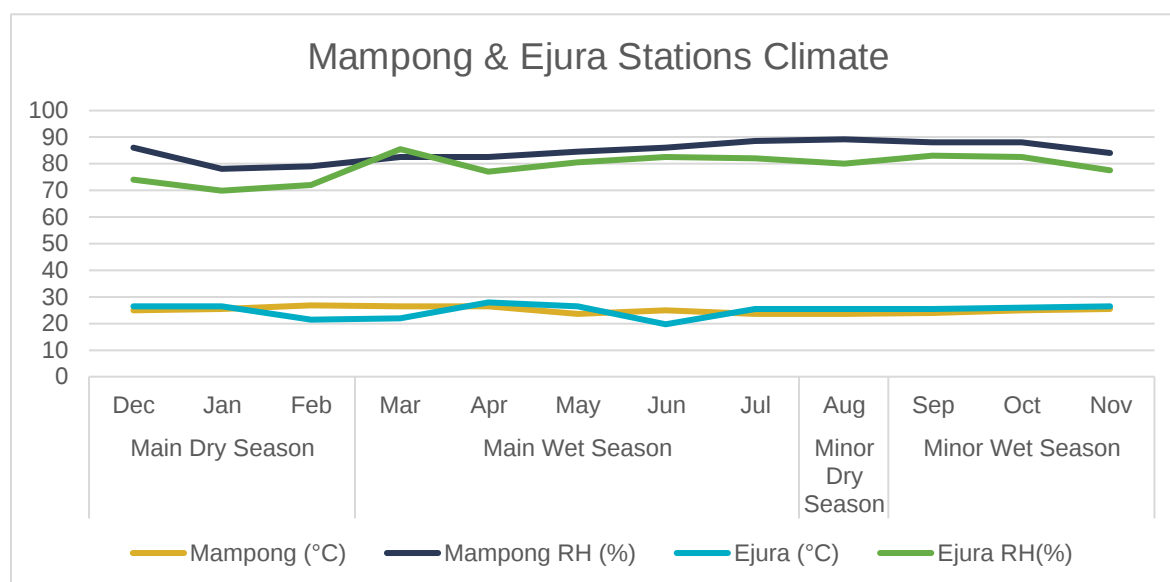
Figure 8. Mean monthly temperatures (°C) and RH (%) for Mampong (Ashanti) and Ejura
