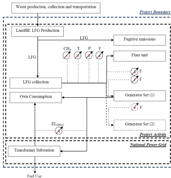
Figure 5: Single Line Diagram
