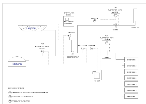
Figure 2 Flow chart of the implemented Project
