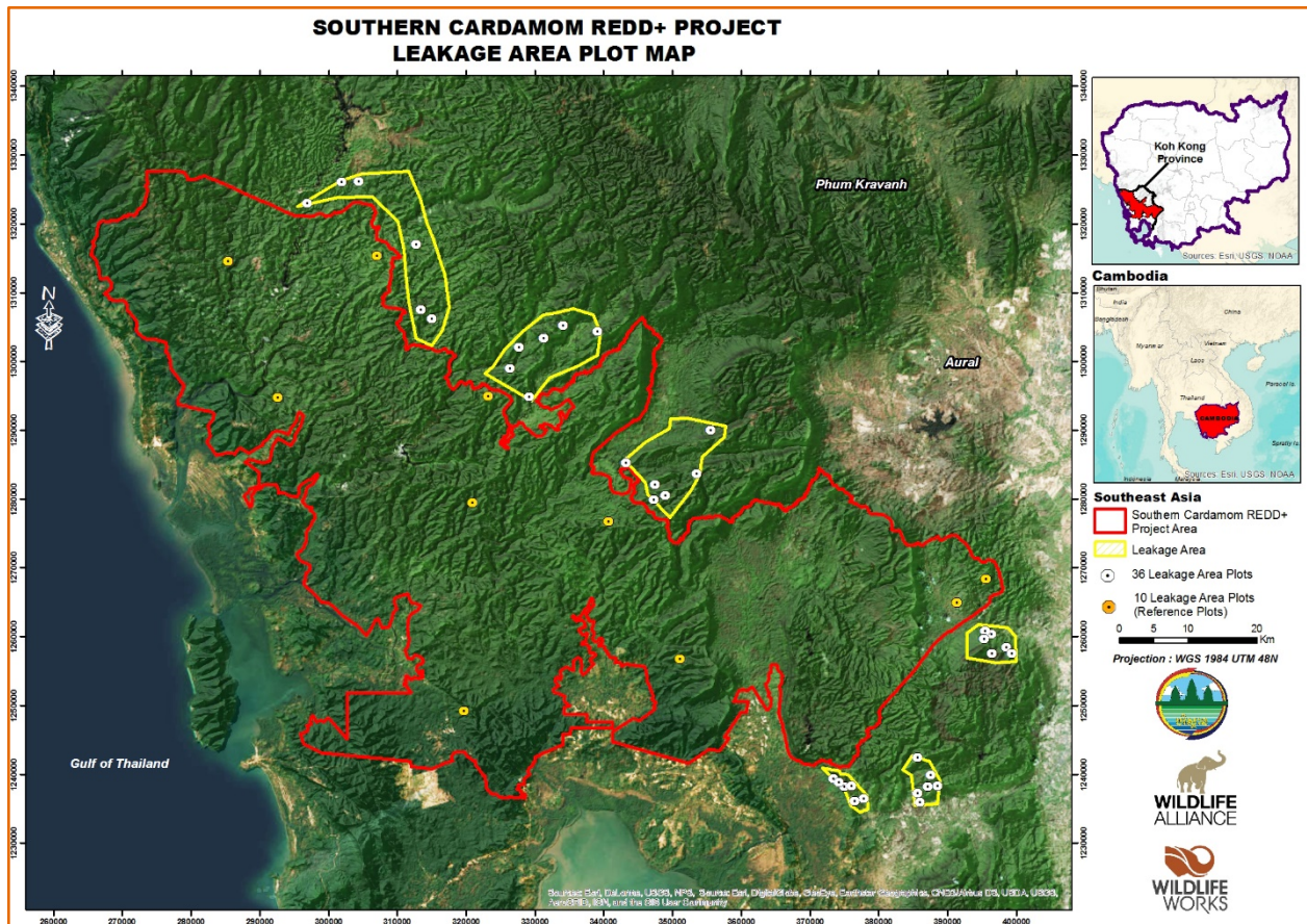
Figure 13: The leakage area for the Southern Cardamoms REDD+ Project is shown. The leakage area sample plot locations are also shown.
