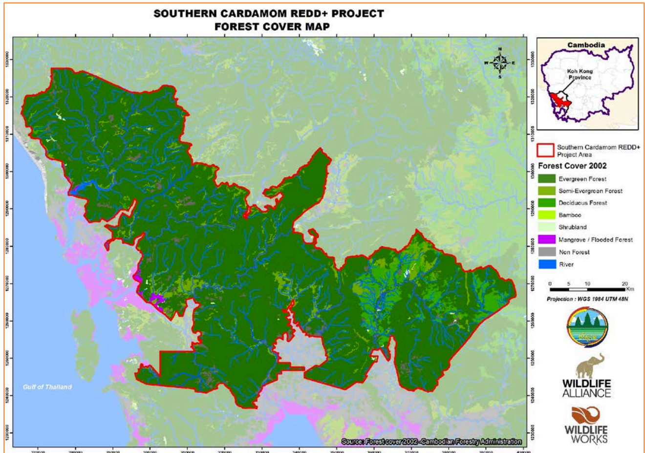
Figure 6: The Project Area, with landcover data indicating forest cover in 2002. This demonstrates compliance with PDR.22, that the PA was forested at least 10 years prior to the Project Start Date.
