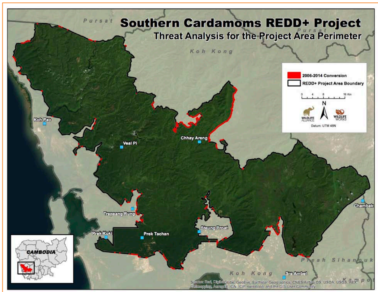
Figure 7: Deforestation analysis for the Project Area perimeter.
