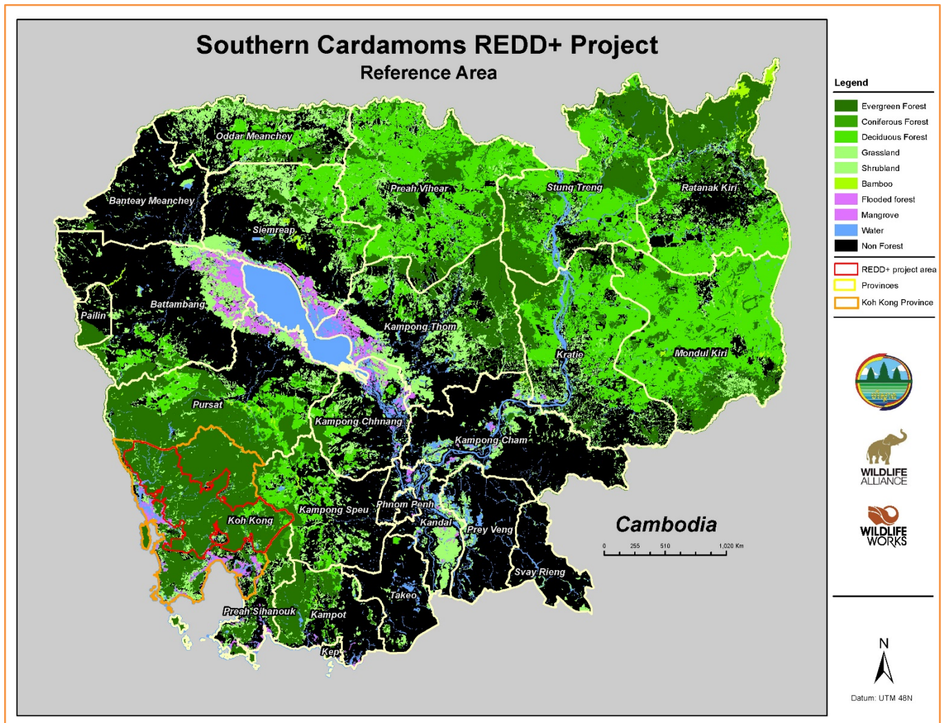
Figure 9: The SCRP reference area in relation to the Project Area.
