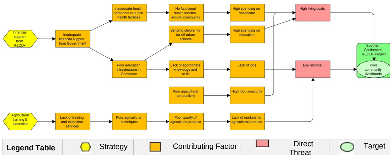
Figure 15: Problem Flow diagrams produced for the Focal Issues during the SIA community workshops in the SCRPP
