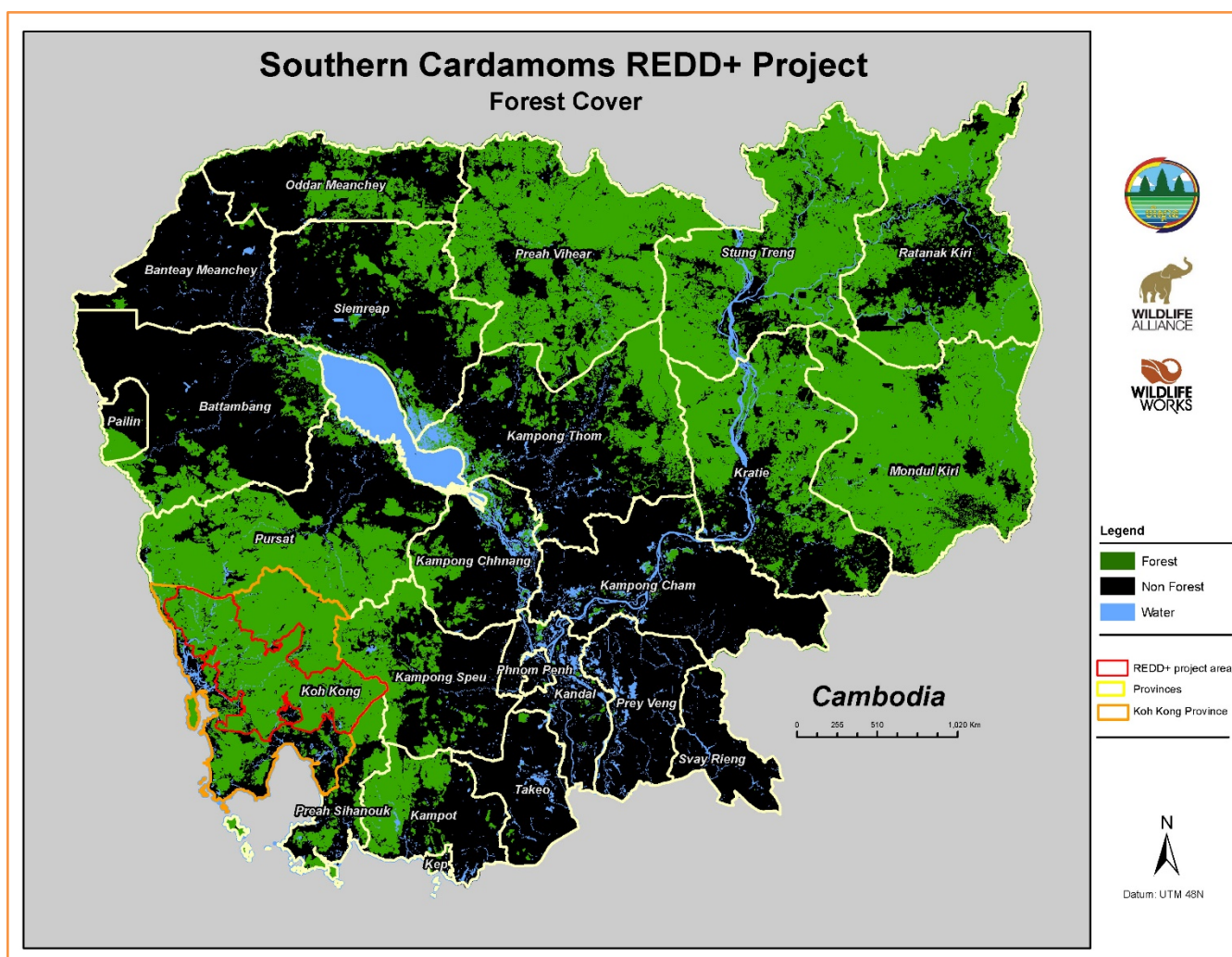
Figure 10: Forest cover in the reference area for the year 2015.
